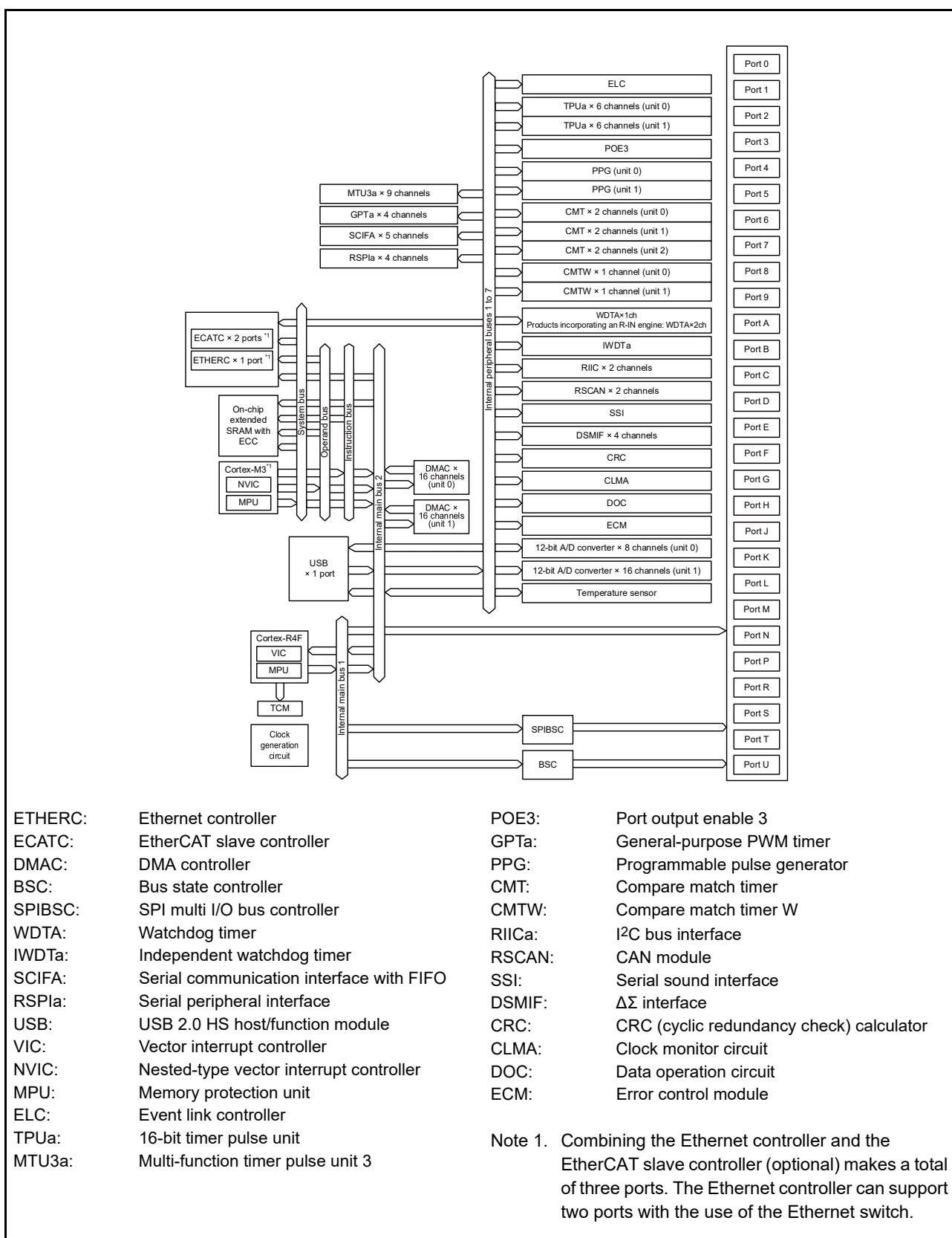
Figure 1.1 Block Diagram
