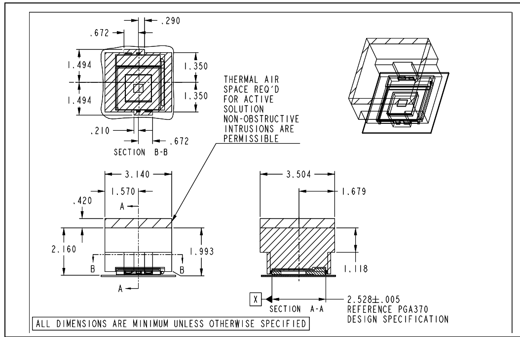
Figure 26. Component Keep-Out
