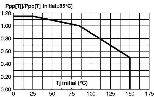
Fig. 3 : Relative variation of peak pulse power versus junction temperature.
