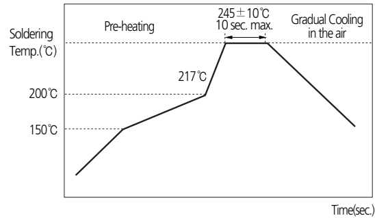
< Reflow Soldering >
