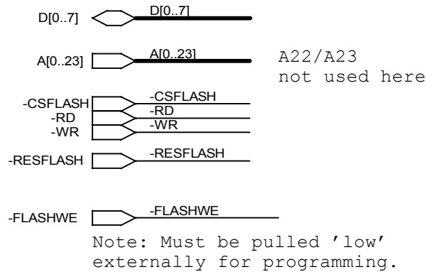
Figure 25. eZ80L92 Module Schematic Diagram, #4 of 9—Flash Device
