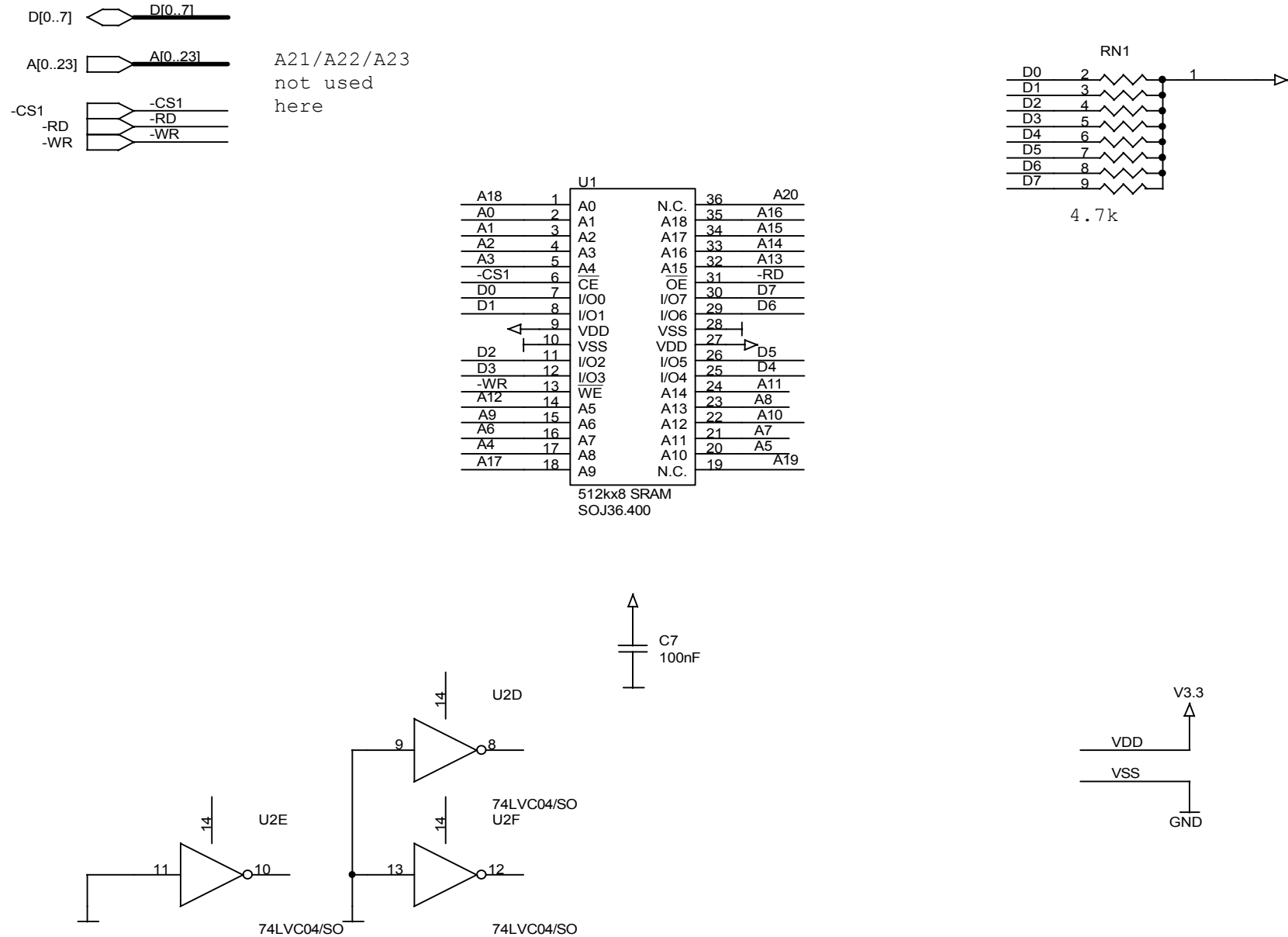
Figure 24. eZ80L92 Module Schematic Diagram, #3 of 9—36-Pin SRAM Device
