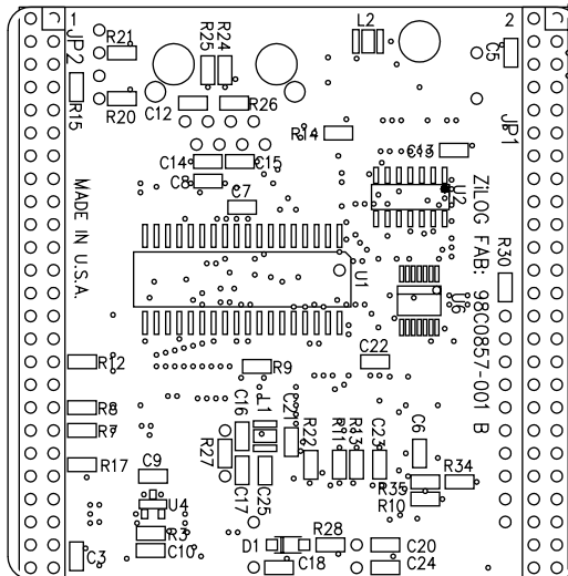
Figure 13. Bottom Layer
