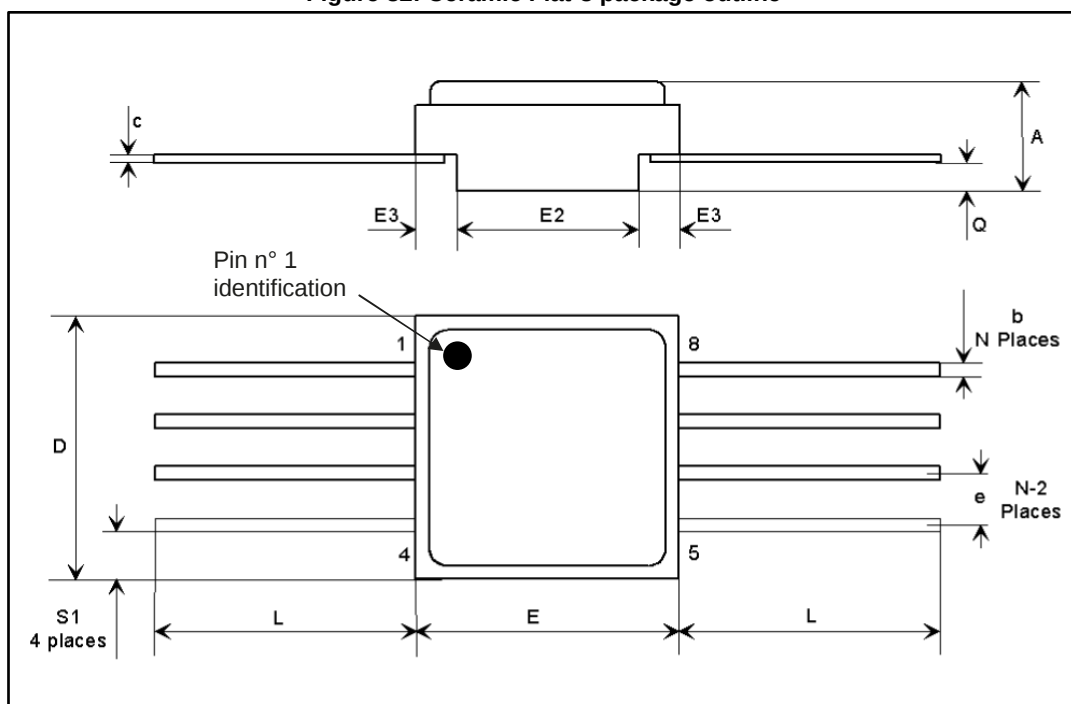
Figure 32: Ceramic Flat-8 package outline
