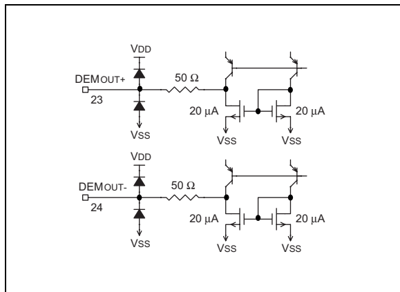
FIGURE 2-11: BLOCK DIAGRAM OF DEMODULATOR OUTPUT PINS
