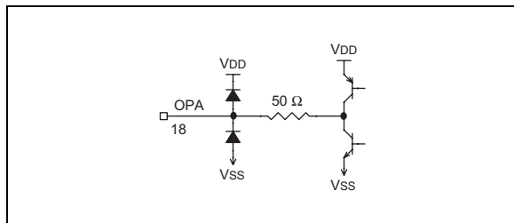
FIGURE 2-13: BLOCK DIAGRAM OF OP AMP OUTPUT PIN
