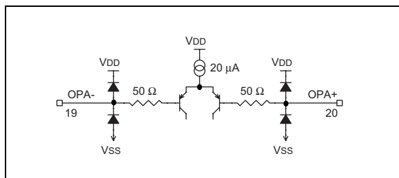
FIGURE 2-12: BLOCK DIAGRAM OF OP AMP INPUT PINS
