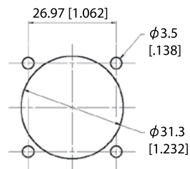
Panel Drilling
