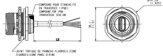
Cable end Type "OPEN" (No connector)
