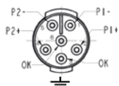
8MF1 P1 and/or P2: 12-48VDC
