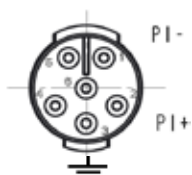
8MF1-704 P1: 12-48VDC 3, 4, 5, 6: Not connected
