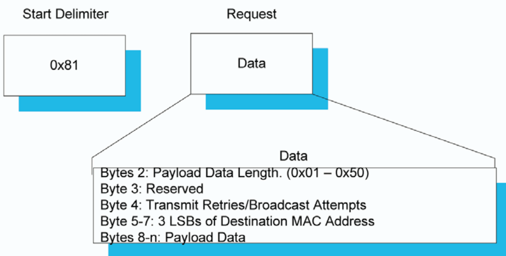
Figure 4: Transmit API Packet Format
