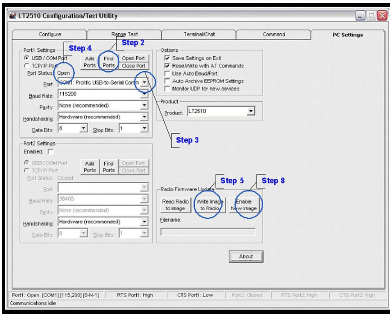
Figure 1: Upgrading firmware in Laird Configuration Utility
