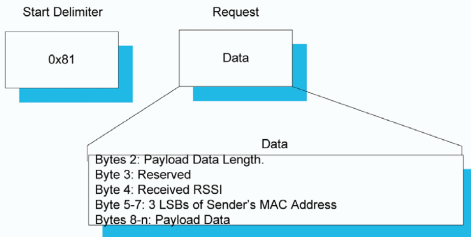
Figure 3: Receive API Packet Format
