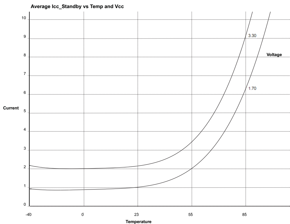
Figure 14-1. Icc3, Supply Current, Standby
