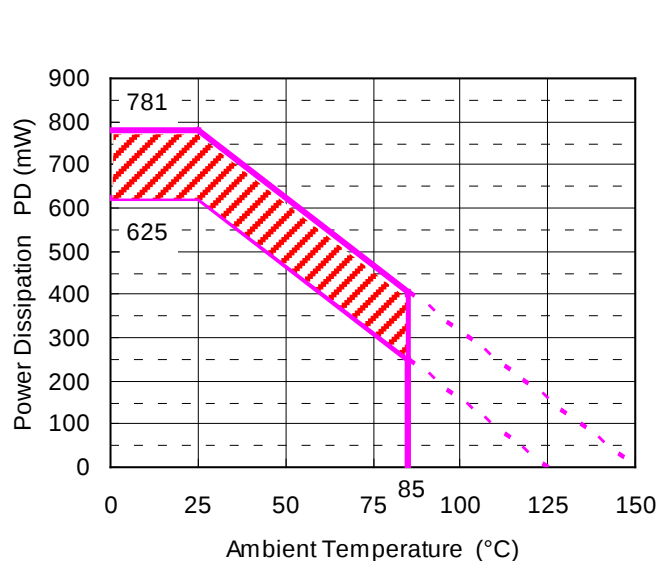
Power Dissipation
