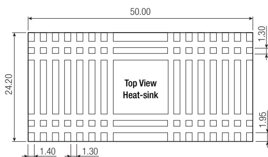
Dimension Drawing (mm) with Heat-sink
