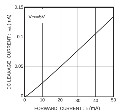
Fig.6 DC leakage current vs. forward current
