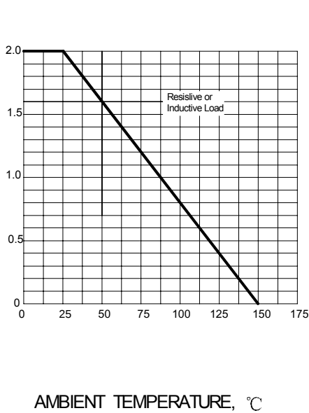
FIG.2 – FORWARD DERATING CURVE
