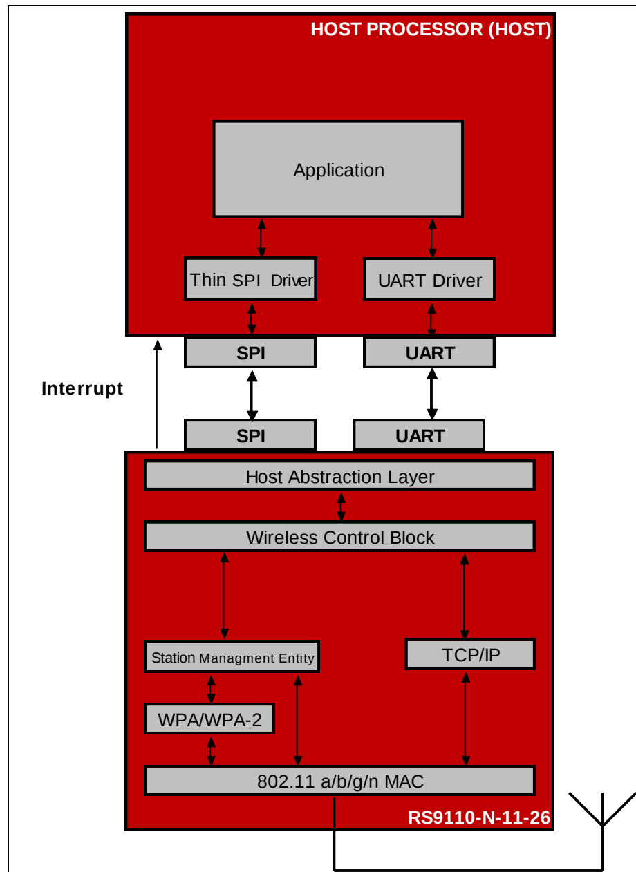
Figure 9: RS9110-N-11-26 Software Architecture Block Diagram
