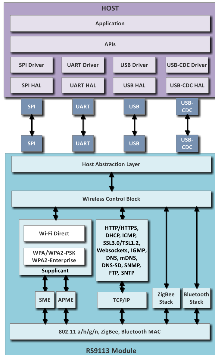
Figure 21: WiSeConnect®/Connect-io-n® Software Architecture
