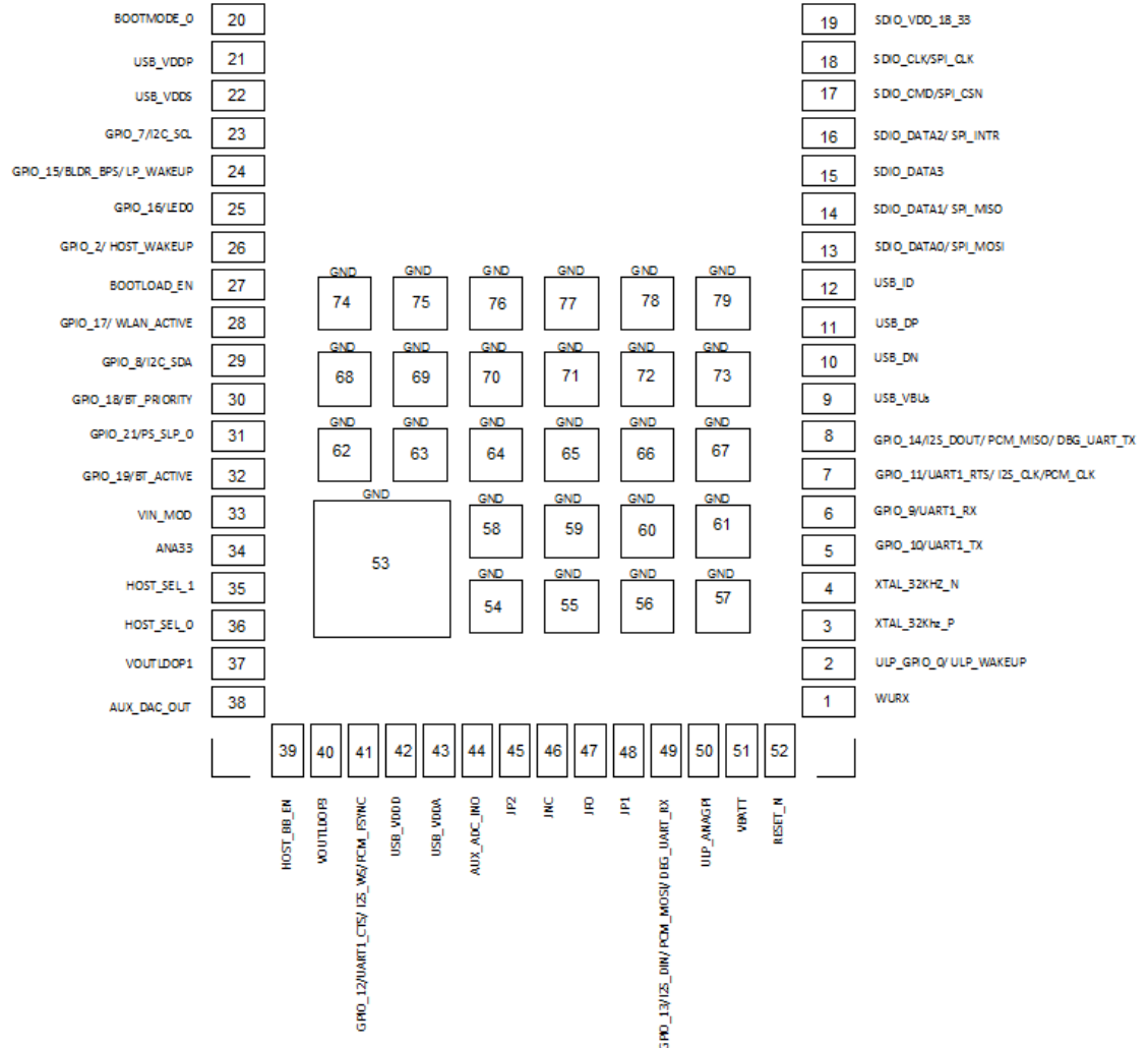
Figure 10: Pinout Diagram of Module with Antenna
