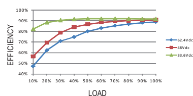
RSD-150C-24
