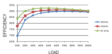
RSD-150D-5
