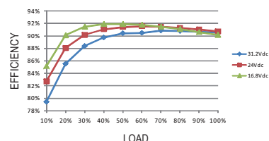
RSD-150C-24
