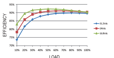
RSD-150C-12
