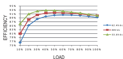
RSD-150C-5
