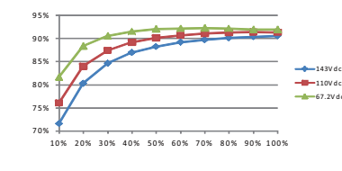
RSD-150D-24
