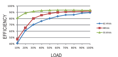
RSD-150C-12
