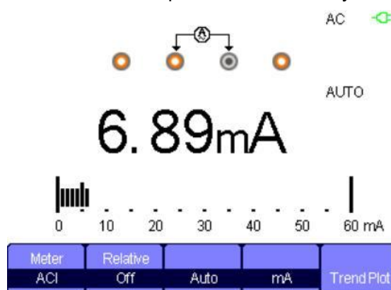
ACI measurement
