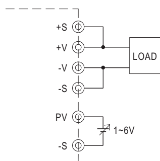
Fig. 3.1 Add on 1~6V external voltage
