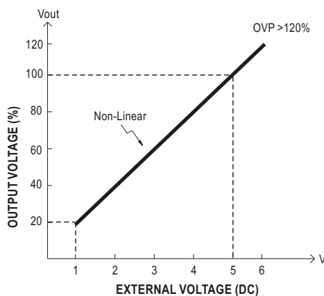
Fig. 3.2 Output voltage trimming
