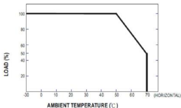
Derating Curve
