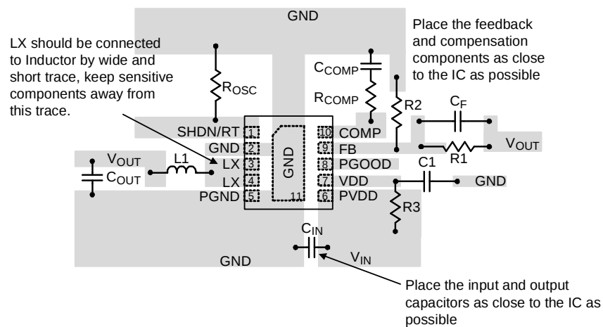
Figure 4. PCB Layout Guide
