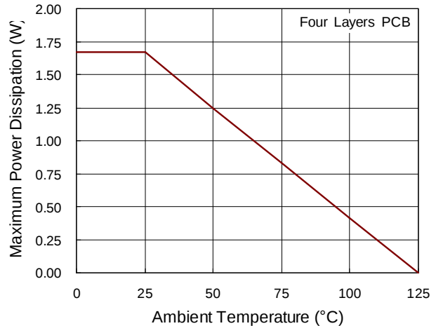
Figure 3. Derating Curves for RT8055B Package
