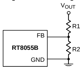
Figure 1. Setting the Output Voltage
