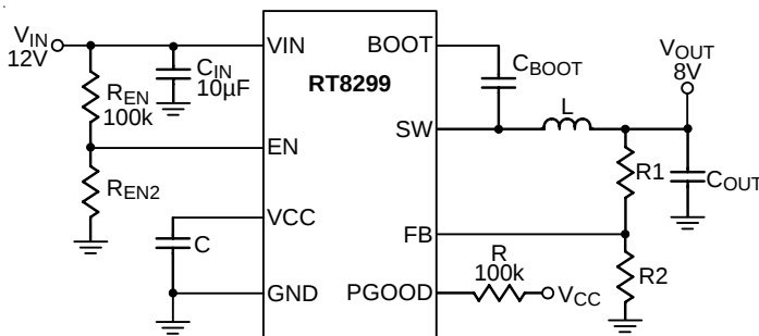
Figure 4. The Resistors can be Selected to Set IC Lockout Threshold
