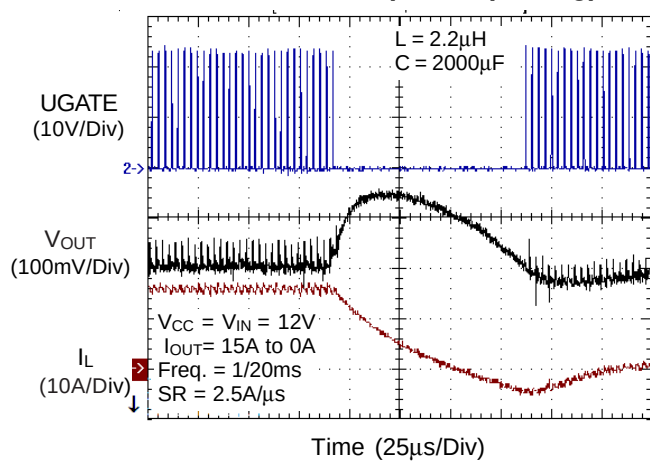
Transient Response (Falling)
