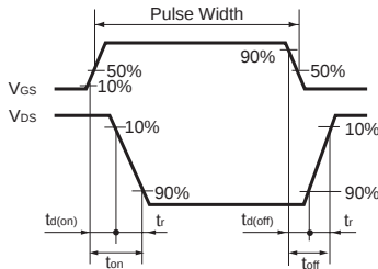
Fig.1-2 Switching Waveforms
