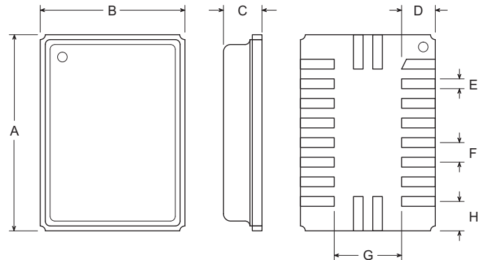
SM-20H Package Drawing
