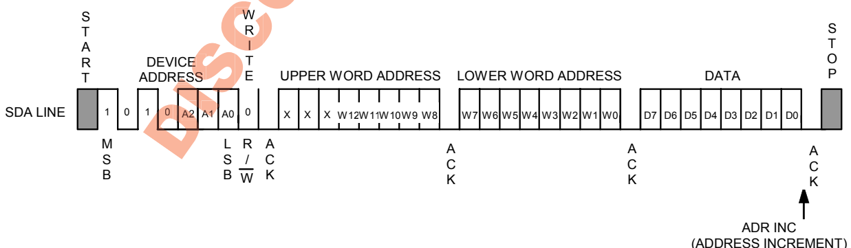
Figure 12 Byte Write
