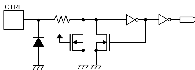
Figure 6 CTRL Pin
