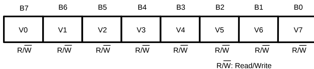
Figure 19 Clock-Correction Register
