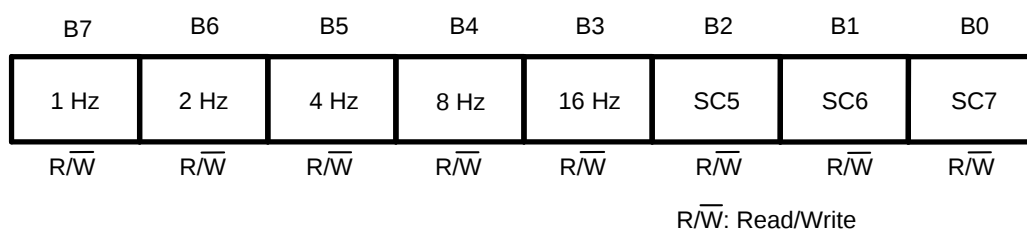
Figure 17 INT2 Register (Data register for output frequency)
