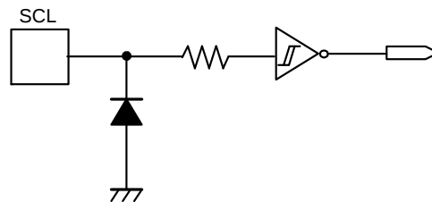
Figure 4 SCL Pin
