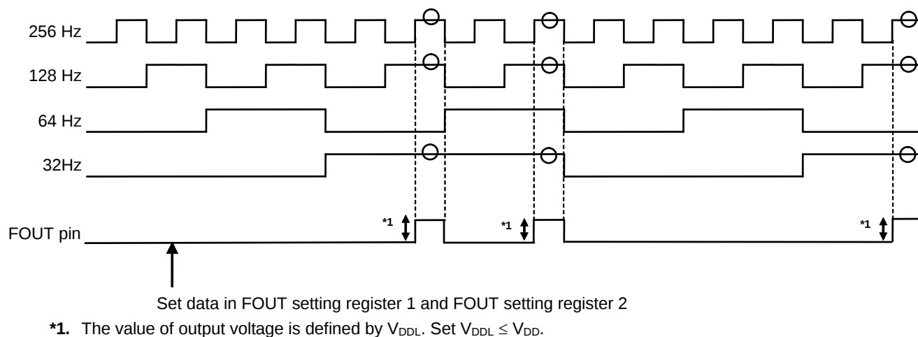
Figure 24 Example of output of clock pulse
