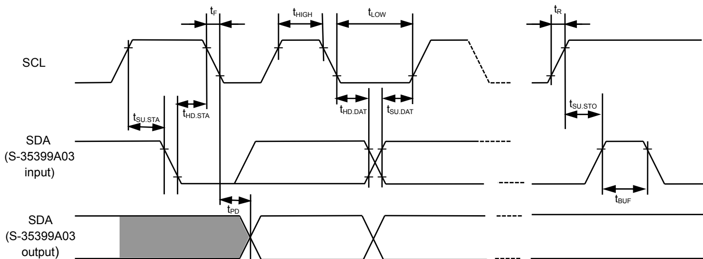
Figure 7 Bus Timing
