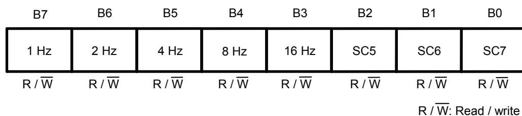
Figure 14 INT2 Register (Data Register for Output Frequency)
