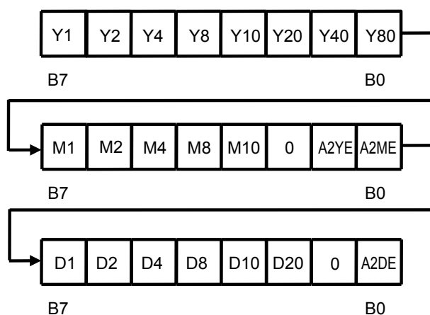
Figure 20 Alarm Expansion Register 1 and Alarm Expansion Register 2
