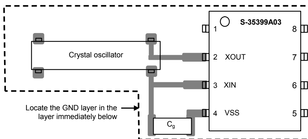
Figure 55 Connection Diagram 2
