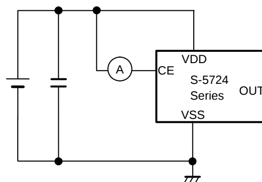
Figure 20 Test Circuit 8
