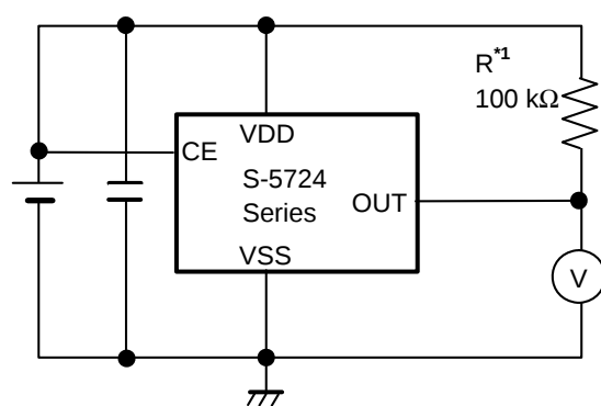
Figure 15 Test Circuit 3
