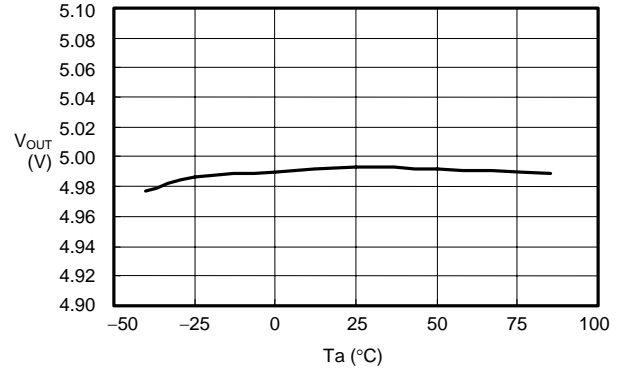
T_a - V_{OUT} S-816A50AMC ( V_{IN}=6 V, I_{OUT}=50 mA)
