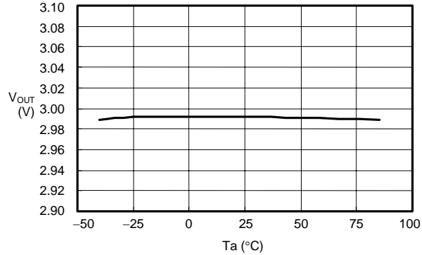
T_a - V_{OUT} S-816A30AMC ( V_{IN}=4 V, I_{OUT}=50 mA)
