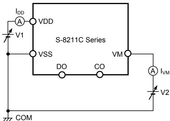
Figure 7 Test Circuit 3
