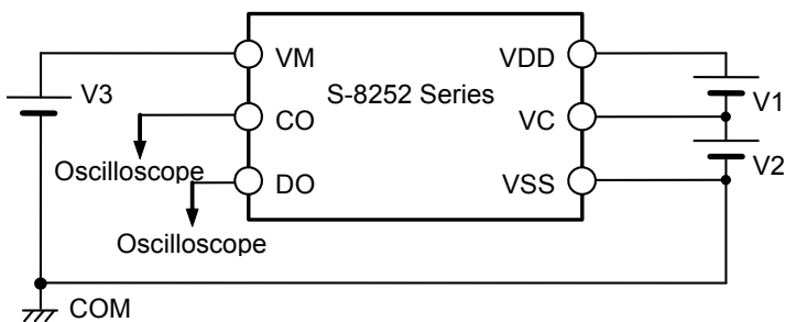
Figure 9 Test Circuit 5
