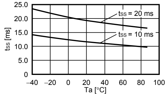
t_{ss} vs. T_a ( V_{IN} = 3.3\text{ V} )
