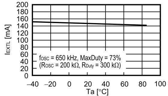
I_{EXTL} vs. T_a ( V_{IN} = 3.3\text{ V} )
