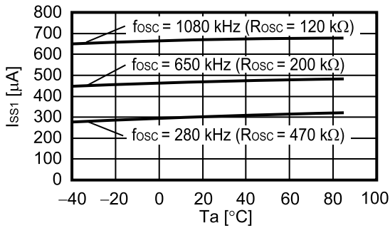
I_{SS1} vs. T_a ( V_{IN} = 3.3\text{ V} )
