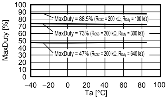
MaxDuty vs. T_a ( V_{IN} = 3.3\text{ V} )
