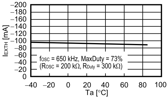
I_{EXTH} vs. T_a ( V_{IN} = 3.3\text{ V} )
