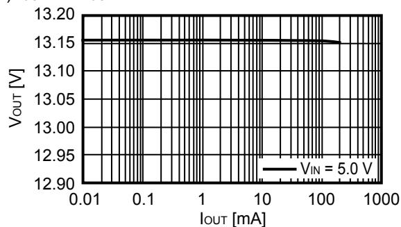
(b) I_{OUT} vs. V_{OUT}
