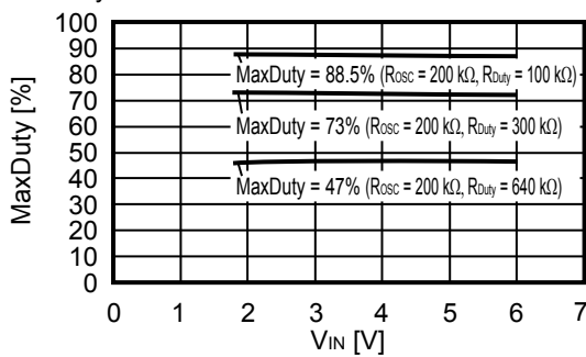
MaxDuty vs. V_{IN}
