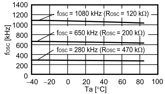
f_{osc} vs. T_a ( V_{IN} = 3.3\text{ V} )
