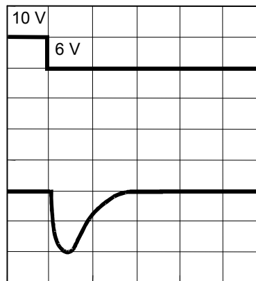
Figure 17 Ringing Waveform of Power Supply Variation (VRO Pin)
