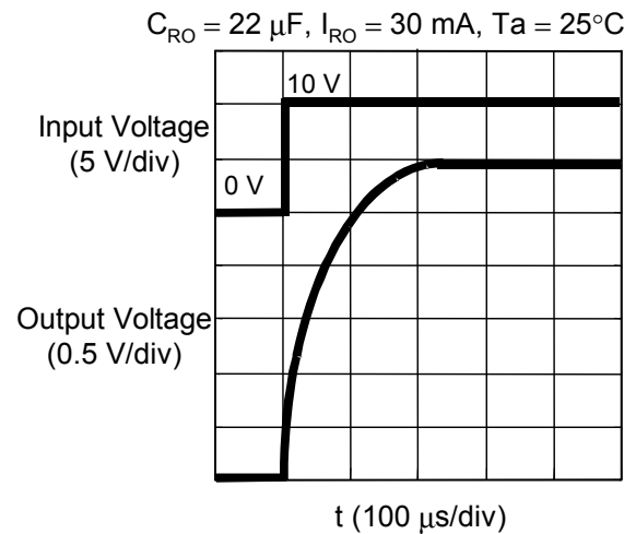
Figure 13 Ringing Waveform of Power Supply Application (VRO Pin)
