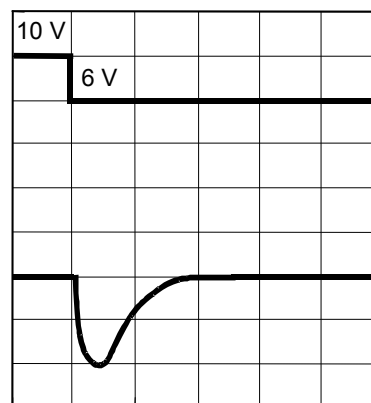
Figure 16 Ringing Waveform of Power Supply Variation (VOUT Pin)
