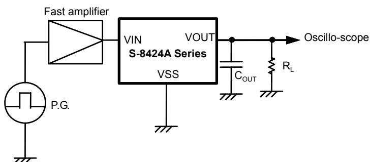
Figure 15 Test Circuit
