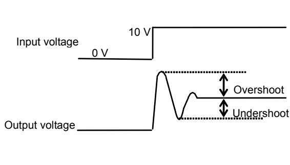
Figure 10 Power Supply Application: 0 V to 10 V Square Wave
