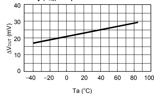
1.12 Load Stability ( V_{RO} ) Temperature Characteristics
