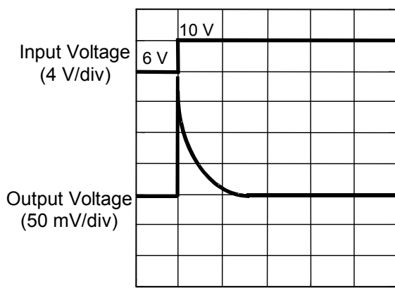
Figure 16 Ringing Waveform of Power Supply Variation (VOUT Pin)
