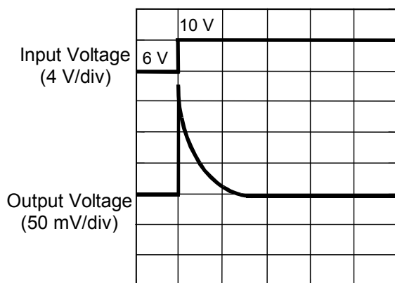
Figure 17 Ringing Waveform of Power Supply Variation (VRO Pin)
