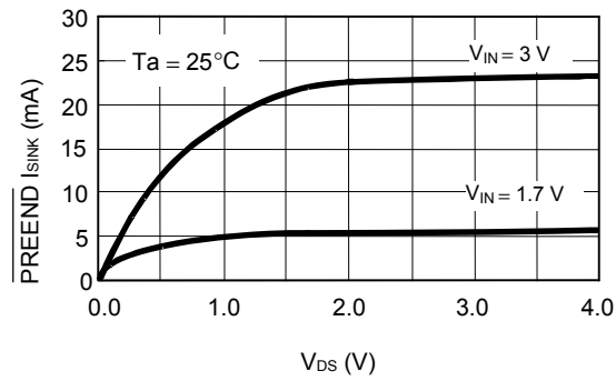
(2) Output current ( I_{SINK} ) characteristics
