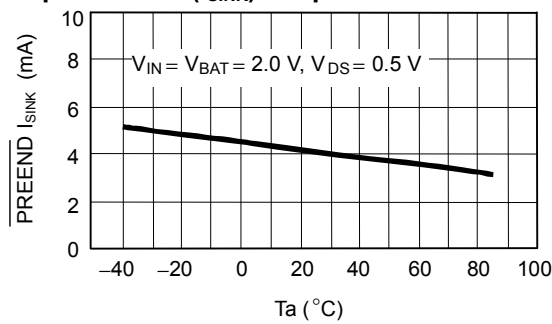
(3) Output current ( I_{SINK} ) temperature characteristics
