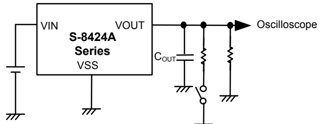
Figure 19 Test Circuit
