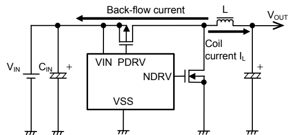
Figure 9 Back-Flow Current
