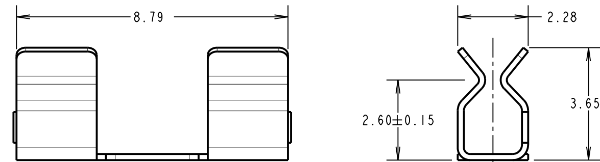
COMPONENT DETAILS
