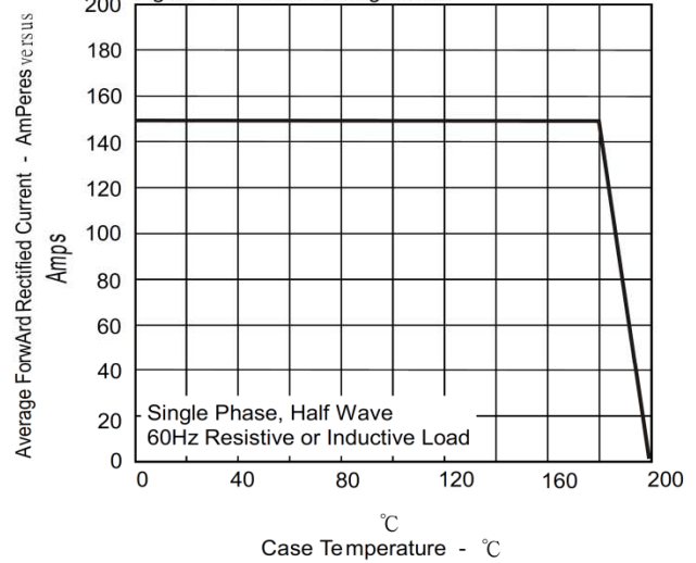
Figur.2-Forward Derating Curve
