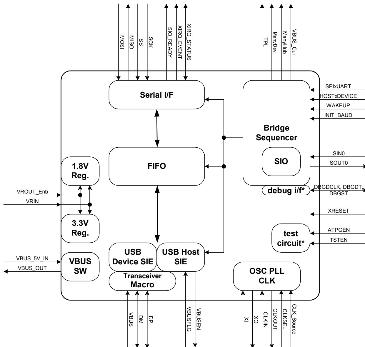
Figure 3.1 Block diagram
