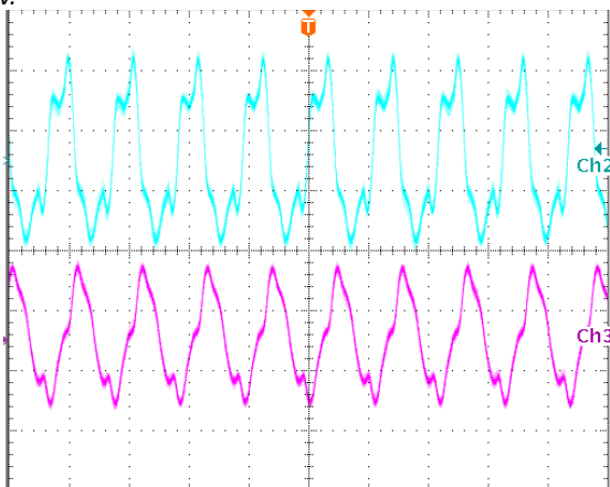
Output voltage ripple at nominal input voltage and max load current Top trace +15V, 10 mV/div, Bottom trace -15V, 20mV/div, 2us/div. Load cap: 10 \mu\text{F} , tantalum capacitor and 1 \mu\text{F} ceramic capacitor. Bandwidth: 20 MHz.
