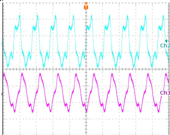
Output voltage ripple at nominal input voltage and max load current Top trace +15V, 10 mV/div, Bottom trace -15V, 20mV/div, 2 \mu s/div. Load cap: 10 \mu F, tantalum capacitor and 1 \mu F ceramic capacitor. Bandwidth: 20 MHz.
