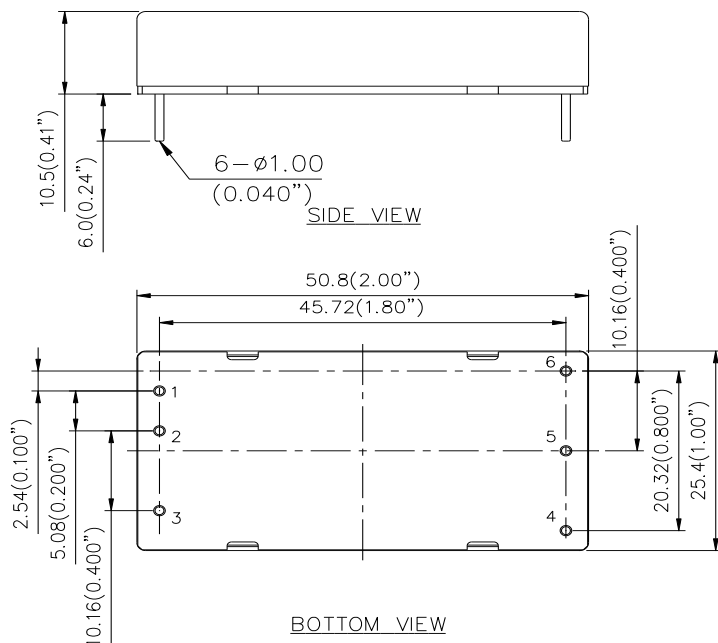
Mechanical Dimensions
