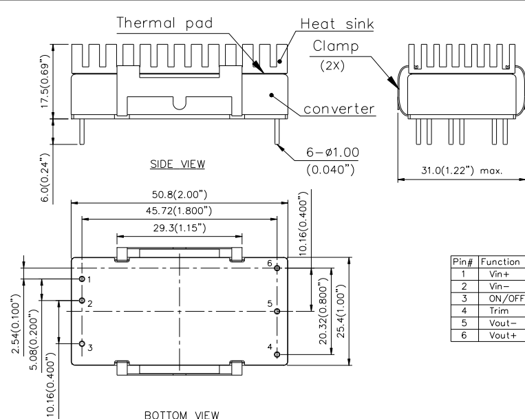
Mechanical Dimensions
