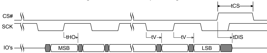
Figure 148. SPI DDR Output Timing
