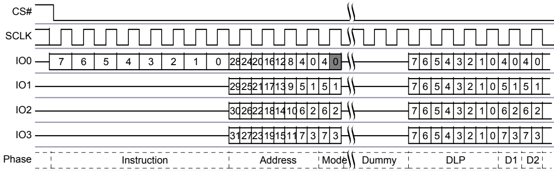
Figure 22. DDR Quad I/O Read Command
