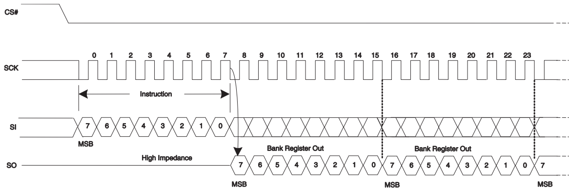
Figure 9.8 Read Bank Register (BRRD) Command
