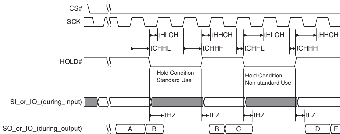
Figure 5.14 Hold Timing
