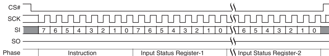
Figure 9.13 Write Registers (WRR 01h) Command Sequence – 24 data bits
