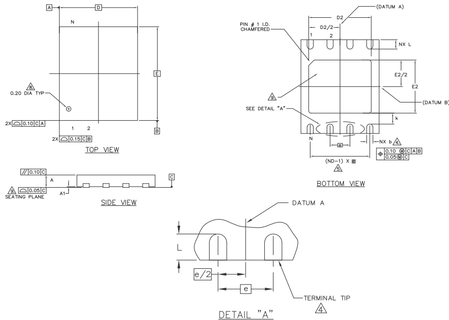
Figure 6.6 WND008 — WSON 8-contact (6 x 5 mm) No-Lead Package
