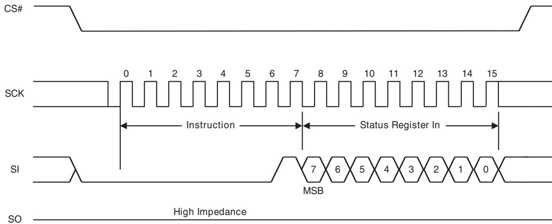
Figure 9.11 Write Registers (WRR) Command Sequence – 8 data bits
