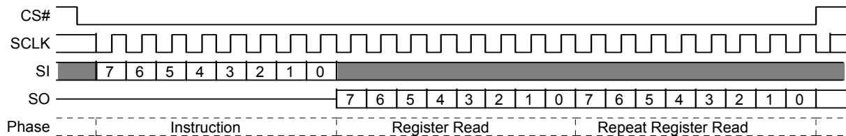
Figure 9.7 Read Configuration Register (RDCR) Command Sequence
