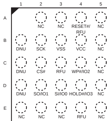
Figure 6.7 24-Ball BGA, 5 x 5 Ball Footprint (FAB024), Top View
