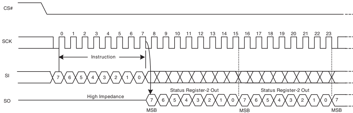
Figure 9.6 Read Status Register 2 (RDSR2) Command
