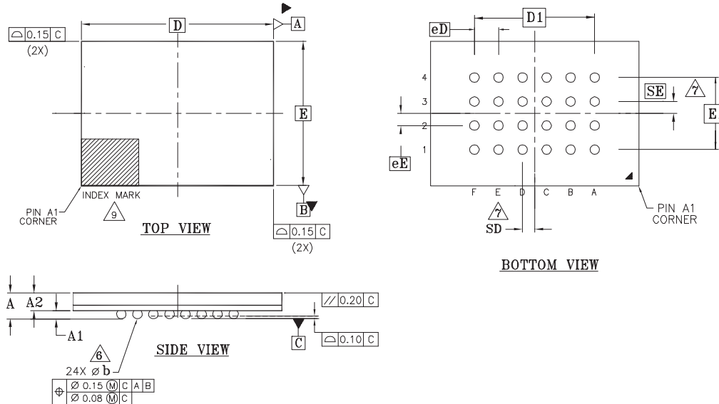
Figure 6.10 FAC024 — 24-ball Ball Grid Array (6 x 8 mm) Package
