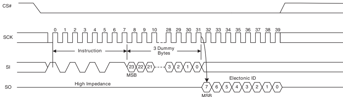
Figure 9.3 Read Electronic Signature (RES) Command Sequence
