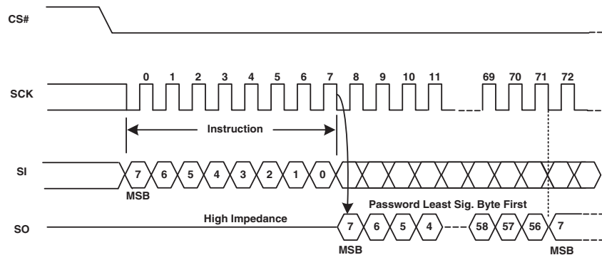
Figure 9.79 Password Read Command Sequence
