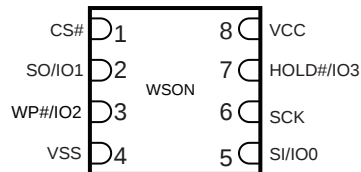
Figure 6.2 Leadless Package (WSON), Top View
