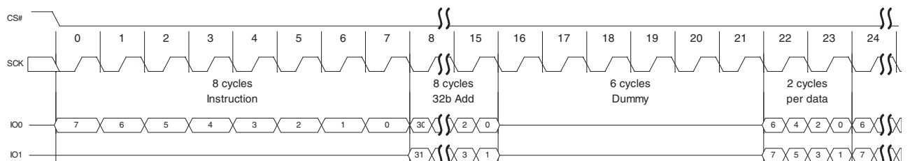
Figure 9.48 DDR Dual I/O Read (4-byte Address, BEh or BDh [ExtAdd=1], HPLC=00b)
