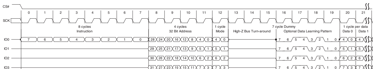
Figure 9.51 DDR Quad I/O Read Initial Access (4-byte Address, EEh or EDh [ExtAdd=1], EHPLC=01b)
