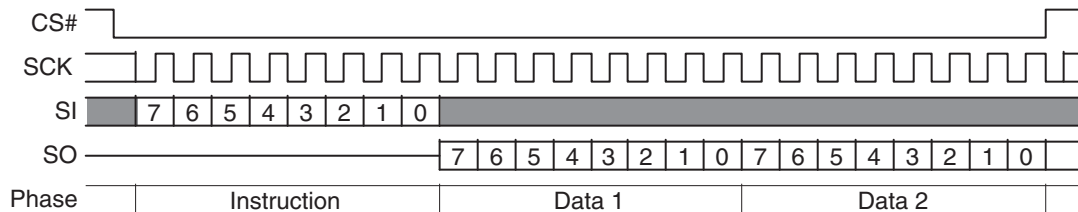
Figure 3.5 Single Bit Wide Output Command
