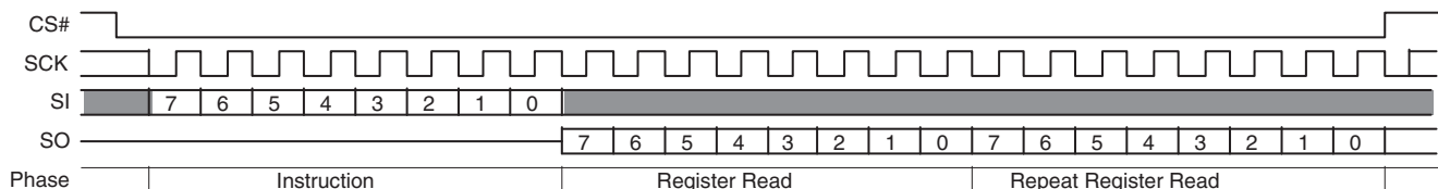
Figure 9.77 PPB Lock Register Read Command Sequence
