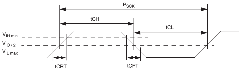
Figure 5.8 Clock Timing
