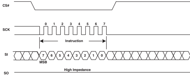
Figure 9.78 PPB Lock Bit Write Command Sequence
