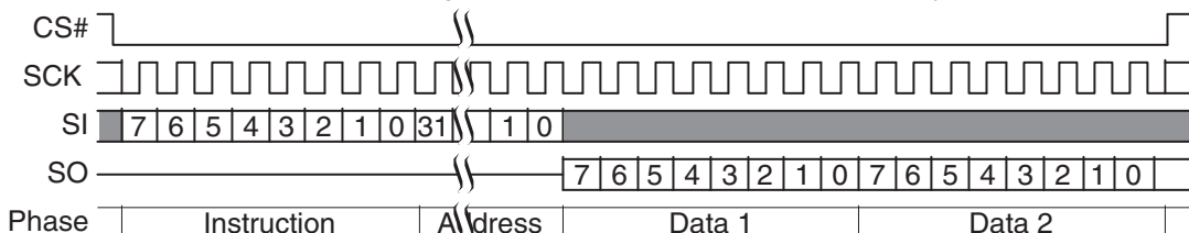
Figure 3.6 Single Bit Wide I/O Command without Latency
