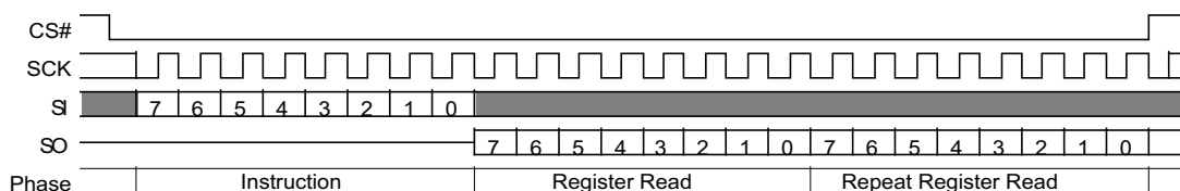
Figure 9.8 Read Bank Register (BRRD 16h) Command
