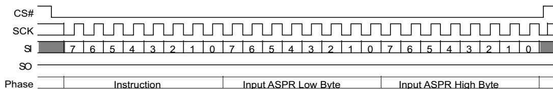
Figure 9.63 ASPP (2Fh) Command
