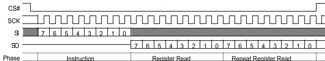
Figure 9.69 PPB Lock Register Read Command Sequence
