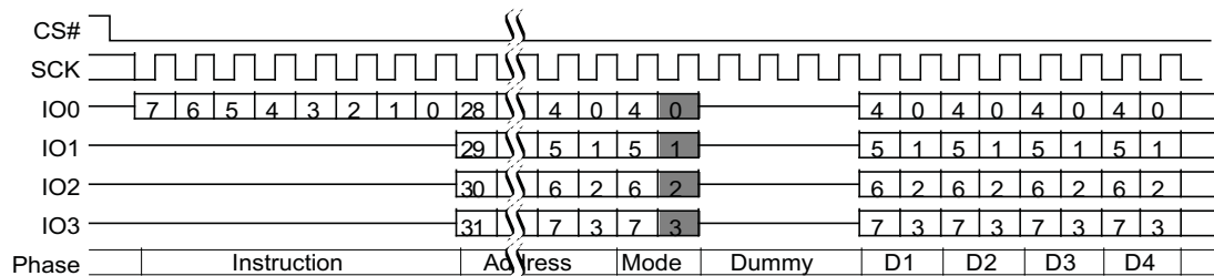
Figure 9.38 Quad I/O Read Command Sequence(4-Byte Address, ECh or EBh [ExtAdd=1], LC=00b)
