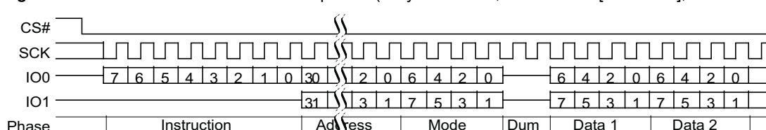
Figure 9.34 Dual I/O Read Command Sequence (4-Byte Address, BCh or BBh [ExtAdd=1], EHPLC=10b)
