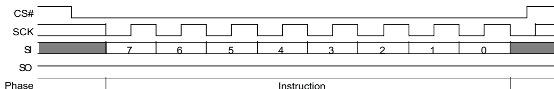
Figure 9.74 Software Reset (RESET F0h) Command Sequence
