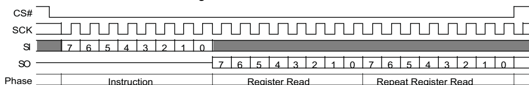
Figure 9.62 ASPRD Command
