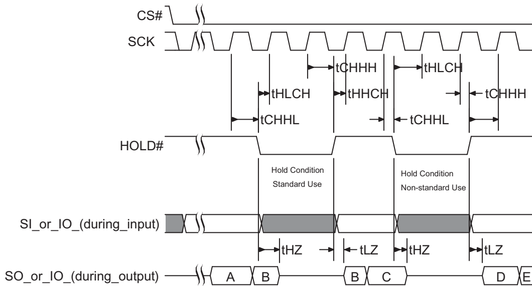
Figure 5.12 Hold Timing
