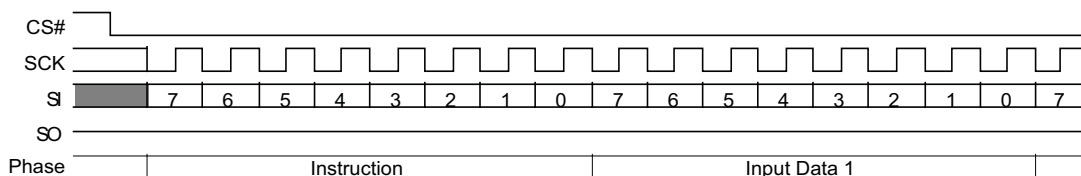
Figure 9.20 AutoBoot Register Write (ABWR) Command
