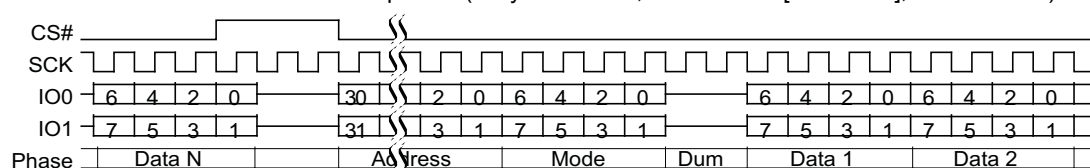
Figure 9.35 Continuous Dual I/O Read Command Sequence (4-Byte Address, BCh or BBh [ExtAdd=1], EHPLC=10b)
