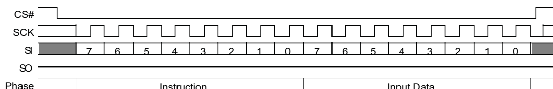
Figure 9.9 Bank Register Write (BRWR 17h) Command
