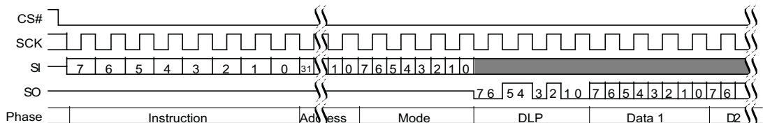
Figure 9.42 DDR Fast Read Initial Access (4-Byte Address, 0Eh or 0Dh [ExtAdd=1], EHPLC=01b)
