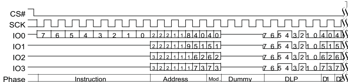
Figure 9.50 DDR Quad I/O Read Initial Access (4-Byte Address, EEh or EDh [ExtAdd=1], EHPLC=01b)
