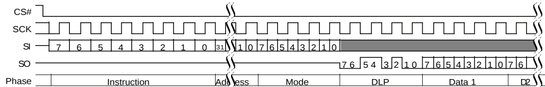
Figure 10.41 DDR Fast Read Initial Access (4-Byte Address, 0Eh or 0Dh [ExtAdd=1, EHPLC=01b])
