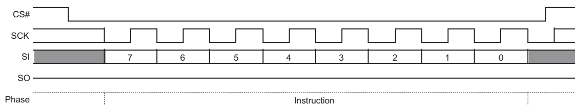
Figure 9.71 Deep Power-Down Command Sequence
