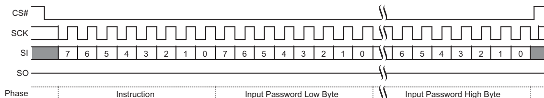
Figure 9.65 Password Program Command Sequence
