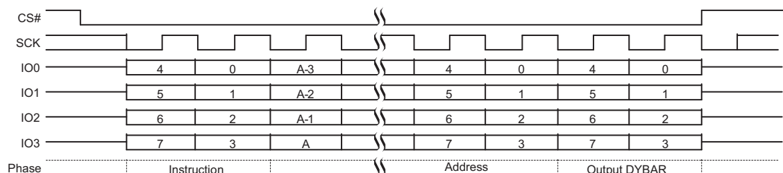
Figure 9.56 DYBRD QPI Mode Command Sequence
