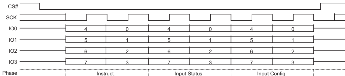
Figure 9.12 Write Registers (WRR) Command Sequence – 16-Data Bits QPI Mode
