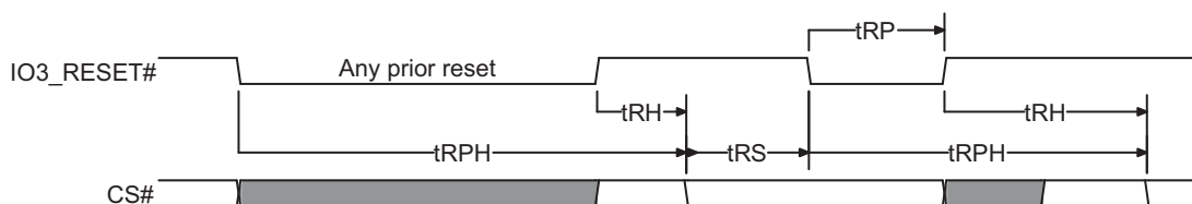
Figure 5.8 Hardware Reset when Quad Mode and IO3 / Reset# are Enabled
