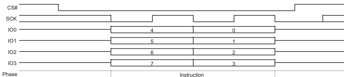
Figure 9.70 Mode Bit Reset Command Sequence QPI Mode
