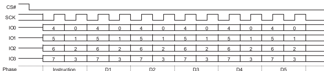
Figure 9.2 Read Identification (RDID) QPI Mode Command
