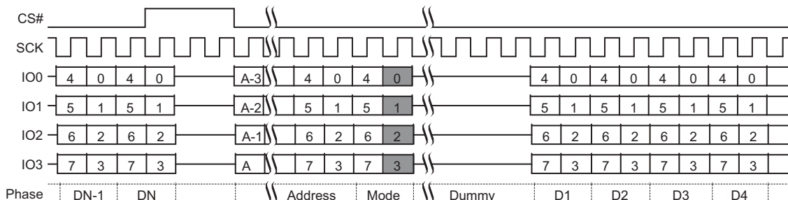
Figure 9.34 Continuous Quad I/O Read Command Sequence (EBh or ECh)
