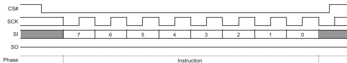
Figure 9.69 Mode Bit Reset Command Sequence
