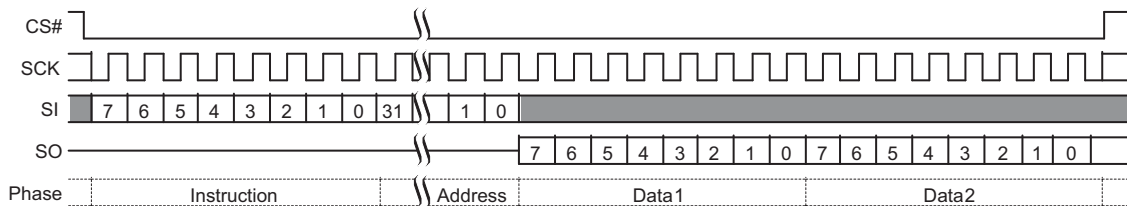
Figure 3.6 Single Bit Wide I/O Command without Latency
