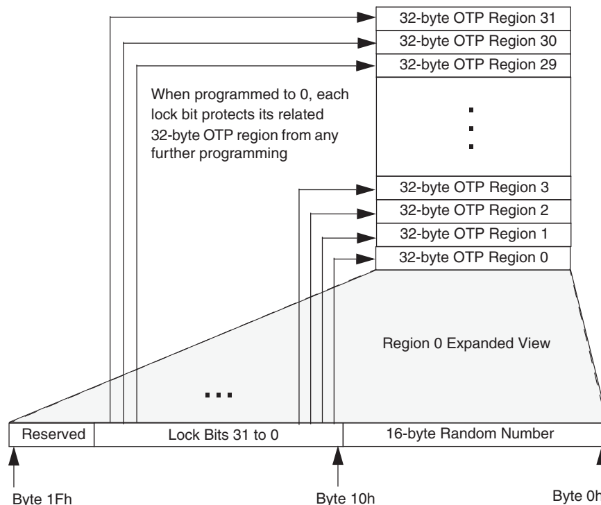
Figure 7.1 OTP Address Space
