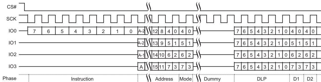
Figure 9.35 DDR Quad I/O Read Initial Access (EDh or EEh)
