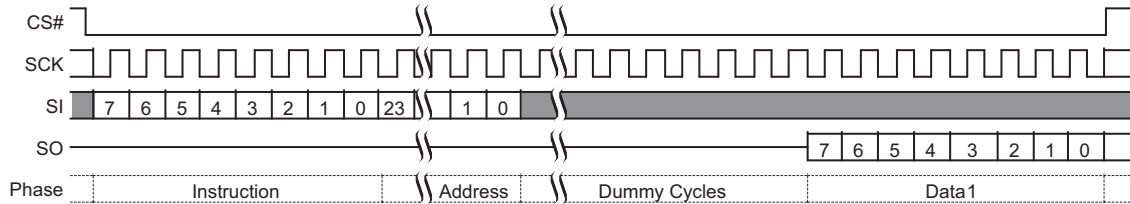
Figure 9.4 RSFDP Command Sequence
