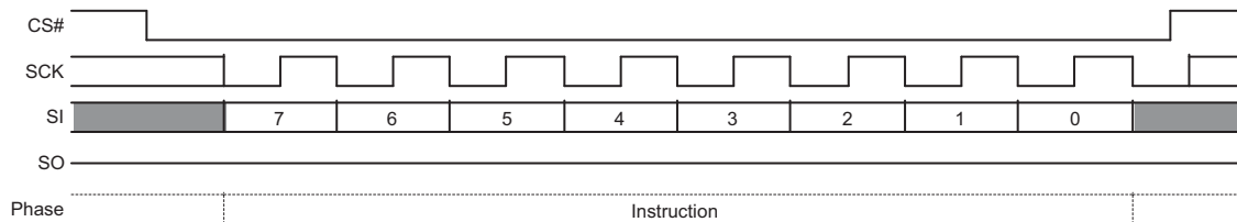
Figure 9.24 Enter 4-Byte Address Mode (4BAM B7h) Command Sequence
