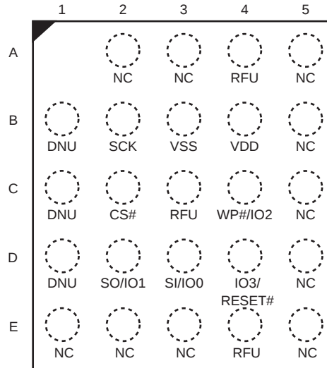
Figure 6.8 24-Ball BGA, 5x5 Ball Footprint (FAB024), Top View
