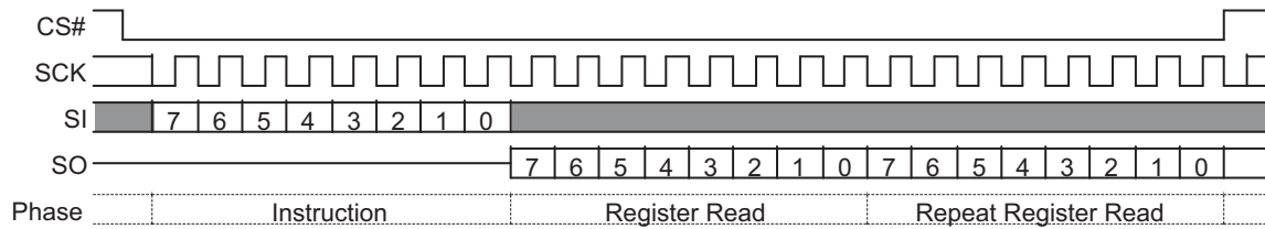
Figure 9.23 DLP Read (DLPRD) Command Sequence
