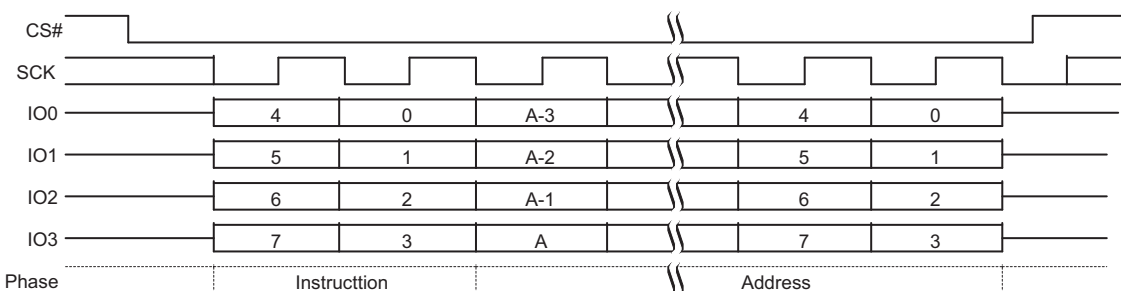
Figure 9.47 EES QPI Mode Command Sequence
