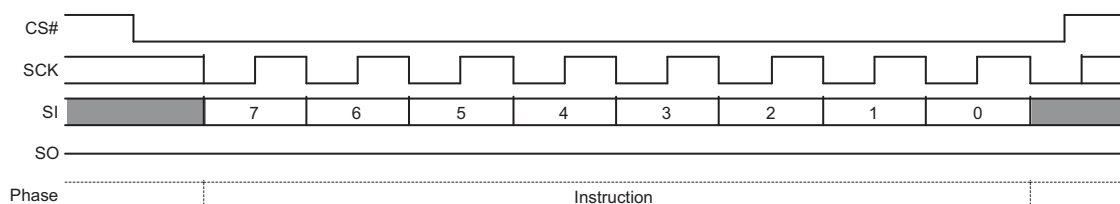
Figure 9.44 Bulk Erase Command Sequence
