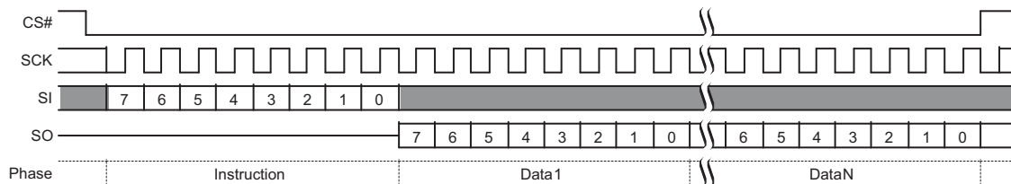
Figure 9.64 Password Read Command Sequence
