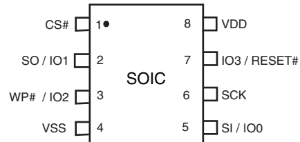
Figure 6.3 8-Pin Plastic Small Outline Package (SOIC8)
