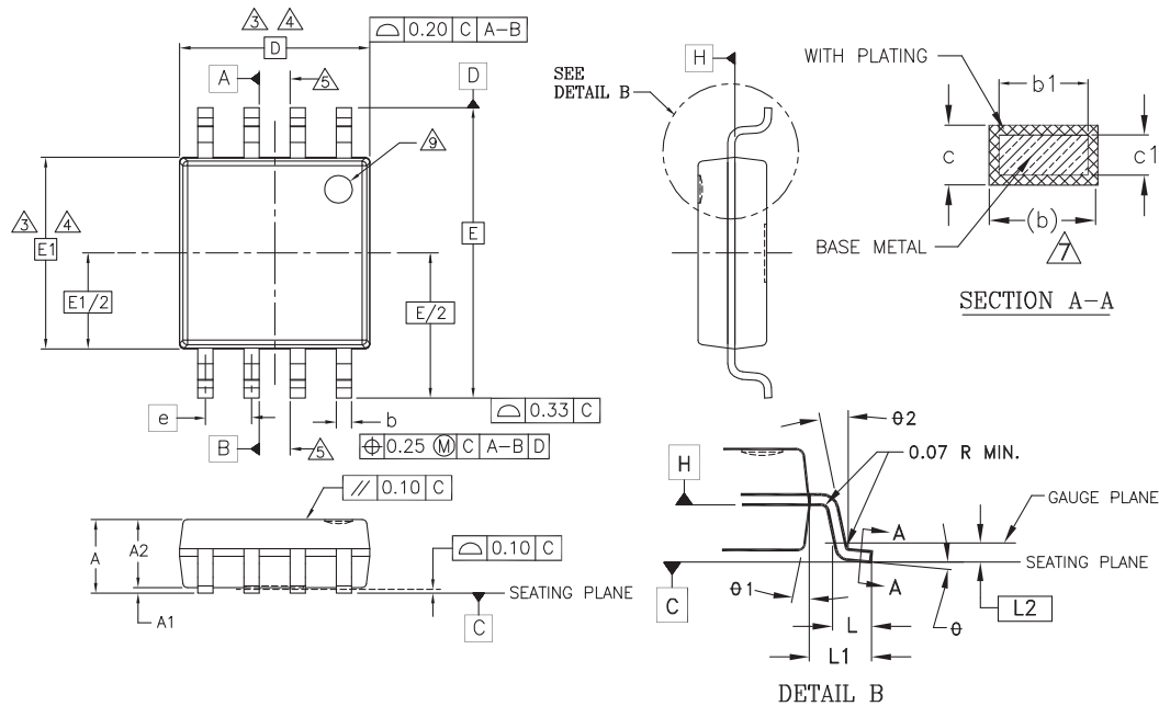
Figure 6.5 SOIC 8-Lead, 208 mil Body Width (SOC008)
