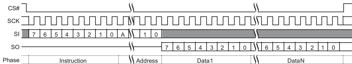
Figure 9.28 Read Command Sequence (3-Byte Address, 03h or 13h)
