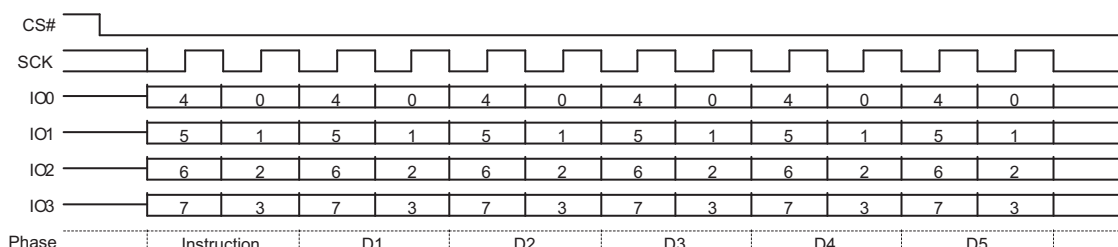
Figure 9.3 Read Quad Identification (RDQID) Command Sequence
