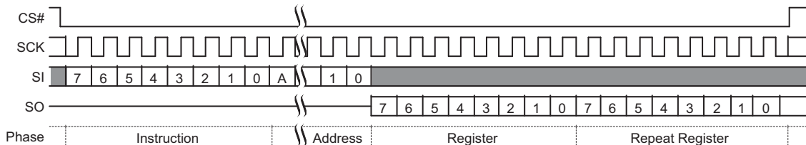
Figure 9.55 DYBRD Command Sequence
