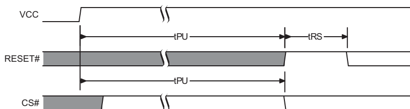
Figure 5.6 POR Followed by hardware reset
