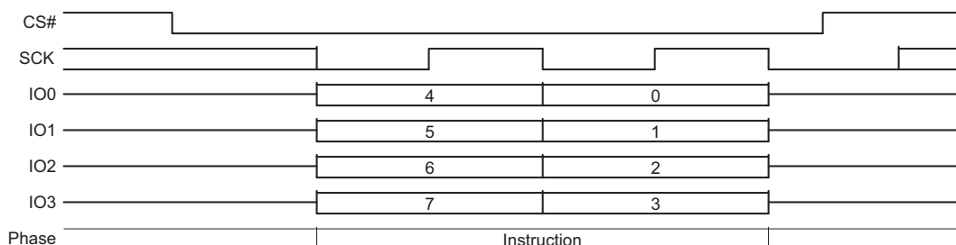
Figure 9.74 RES Command Sequence QPI Mode
