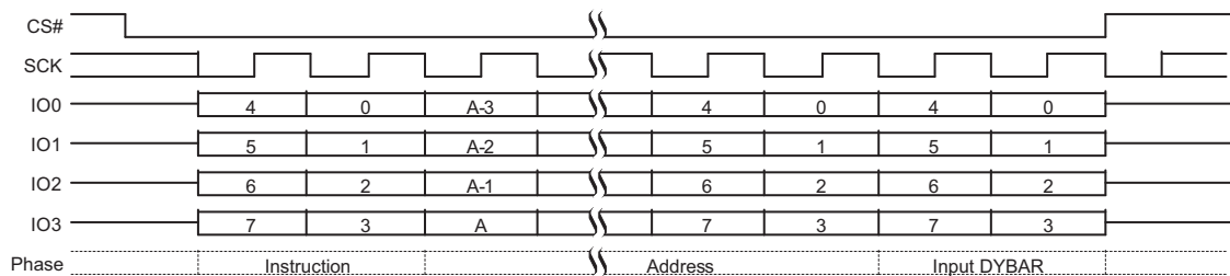
Figure 9.58 DYBWR QPI Mode Command Sequence
