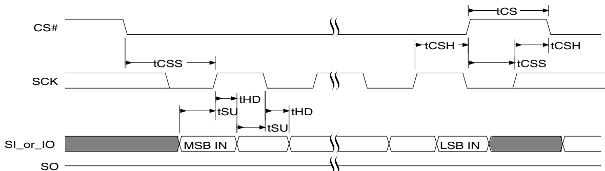
Figure 5.14 SPI DDR Input Timing
