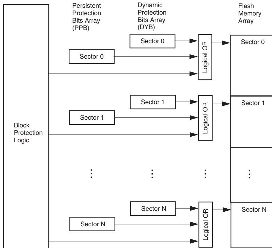
Figure 8.1 Sector Protection Control
