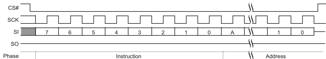
Figure 9.60 PPBP Command Sequence
