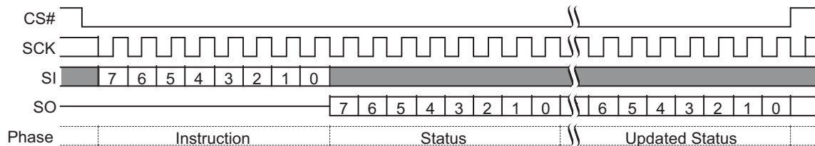
Figure 9.6 Read Status Register 1 (RDSR1) Command Sequence
