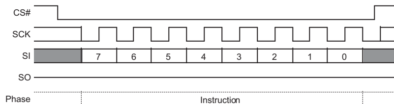
Figure 9.67 Software Reset Command Sequence
