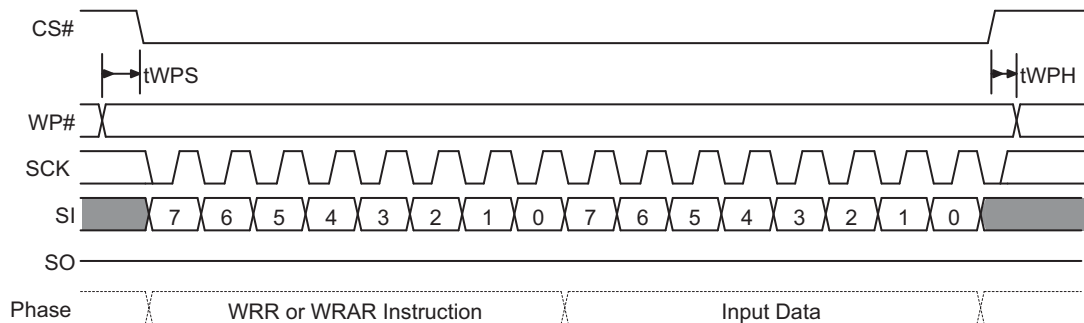
Figure 5.13 WP# Input Timing
