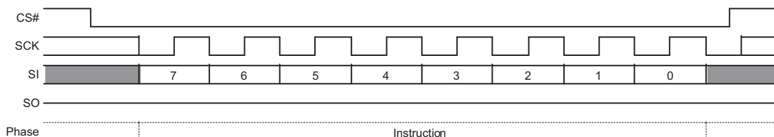
Figure 9.49 Program or Erase Suspend Command Sequence
