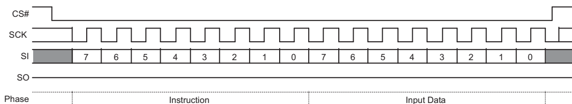
Figure 9.27 Set Burst Length Command Sequence
