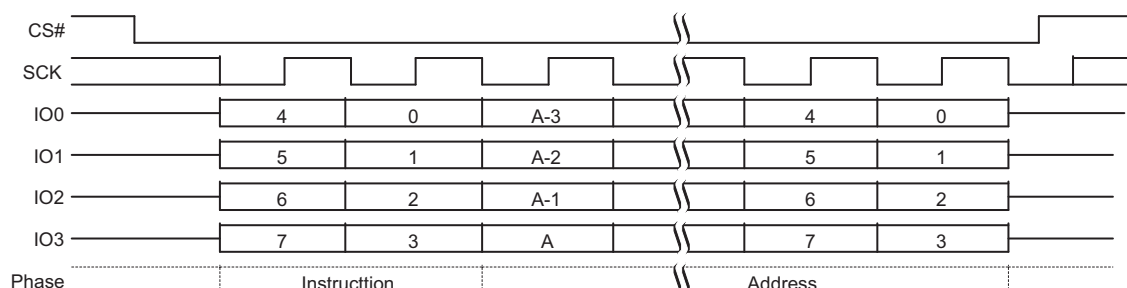
Figure 9.43 Sector Erase (SE D8h or 4SE DCh) QPI Mode Command Sequence
