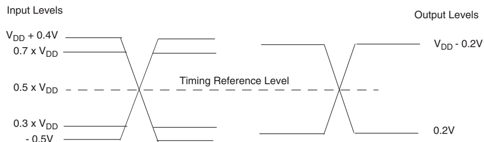
Figure 5.3 Input, Output, and Timing Reference Levels
