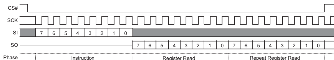
Figure 9.62 PPB Lock Register Read Command Sequence
