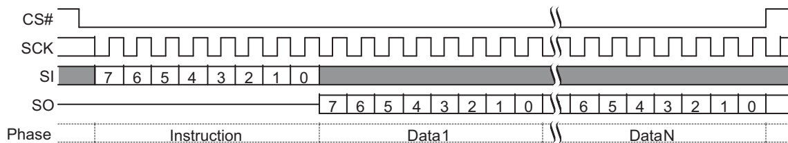
Figure 9.1 Read Identification (RDID) Command Sequence
