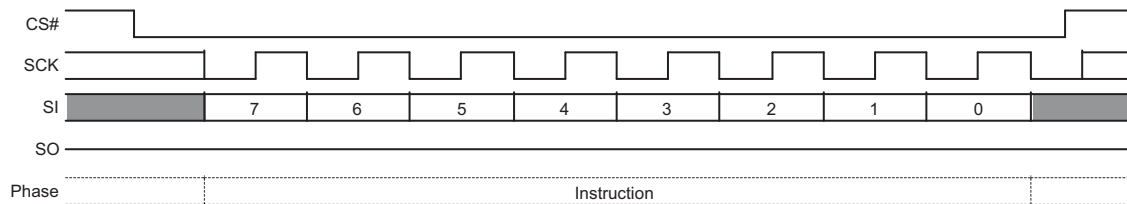
Figure 9.15 Write Disable (WRDI) Command Sequence
