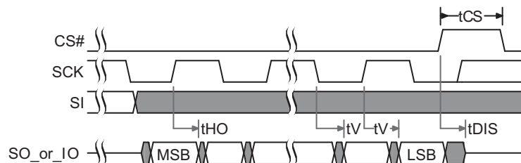
Figure 5.15 SPI DDR Output Timing
