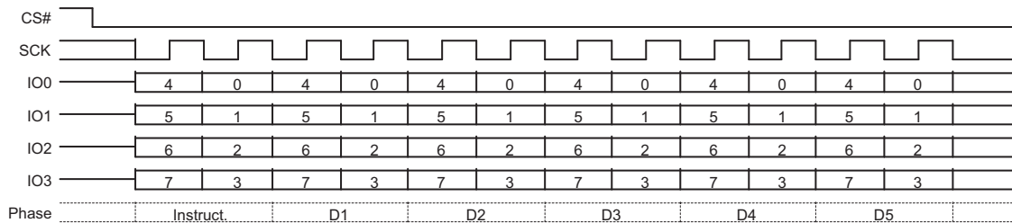
Figure 9.7 Read Status Register 1 (RDSR1) QPI Mode Command
