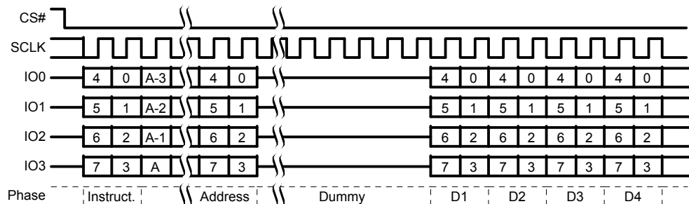
Figure 9.20 ECCRD (19h) or 4EECRD (18h), QPI Mode, Command Sequence
