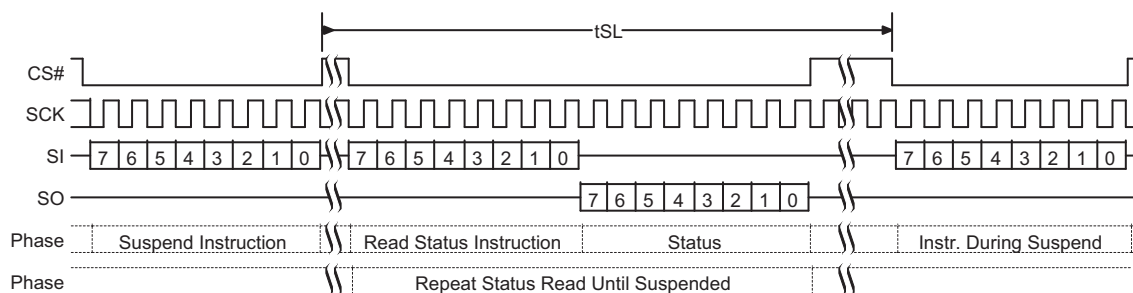
Figure 9.48 Program or Erase Suspend Command Sequence
