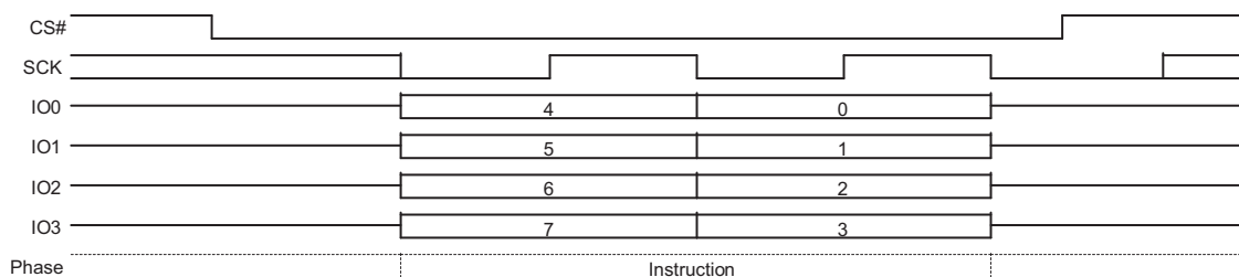
Figure 9.45 Bulk Erase Command Sequence QPI Mode
