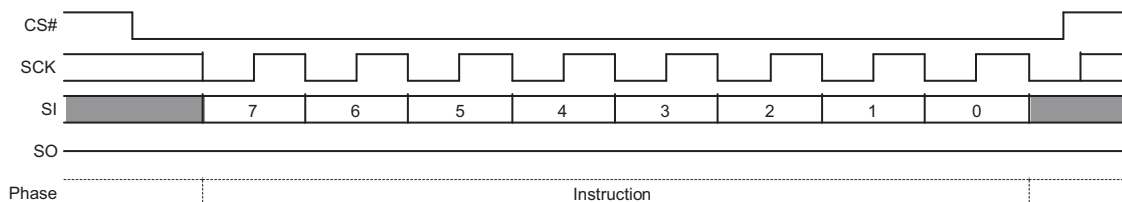
Figure 9.73 Release from Deep Power-Down Command Sequence
