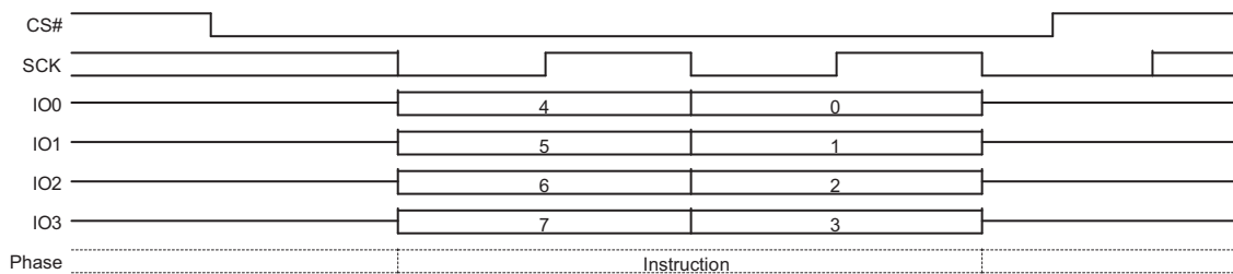
Figure 9.16 Write Disable (WRDI) Command Sequence QPI Mode
