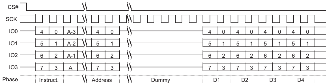
Figure 9.26 Read Any Register, QPI Mode, Command Sequence
