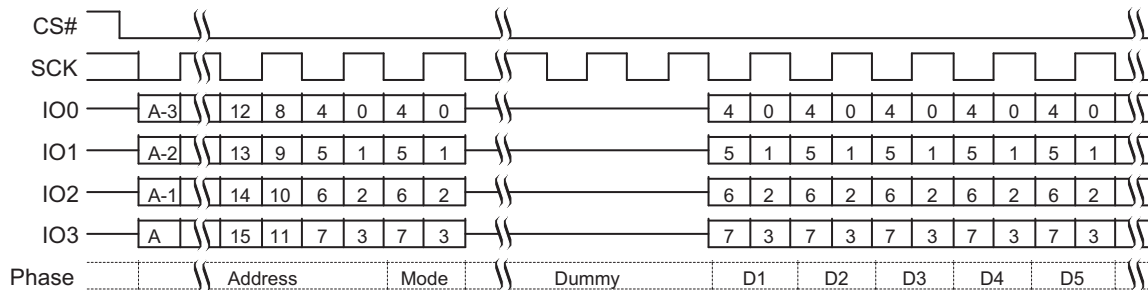
Figure 9.36 Continuous DDR Quad I/O Read Subsequent Access (EDh or EEh)
