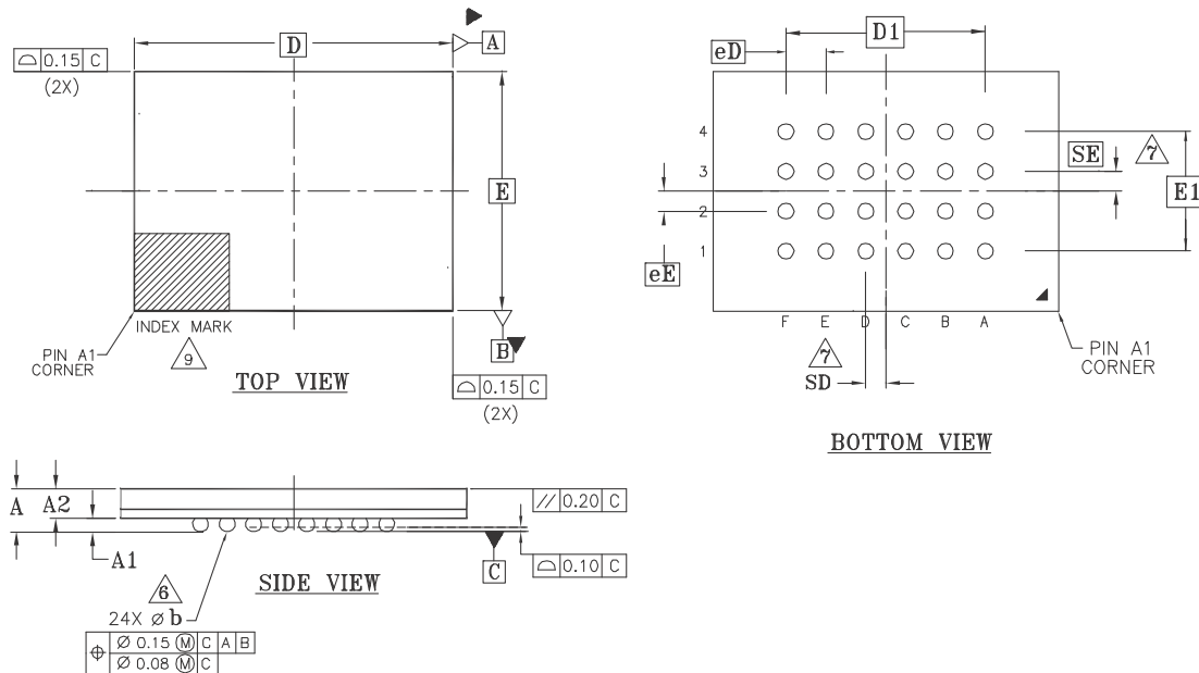
Figure 6.11 Ball Grid Array 24-Ball 6 x 8 mm (FAC024)
