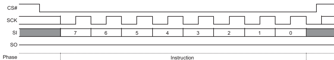
Figure 9.61 PPB Erase Command Sequence
