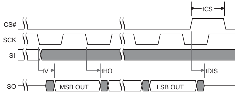
Figure 5.12 SPI SDR MIO Timing
