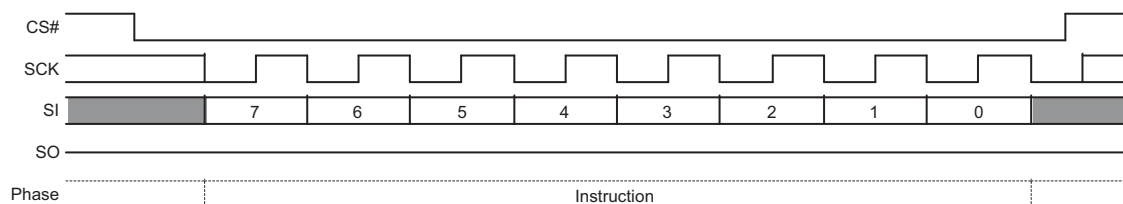
Figure 9.63 PPB Lock Bit Write Command Sequence
