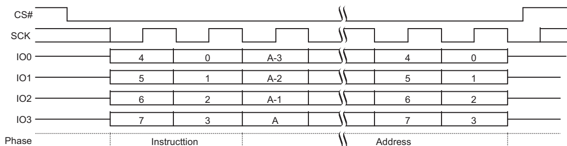
Figure 9.41 Parameter Sector Erase (P4E 20h or 4P4E 21h) QPI Mode Command Sequence
