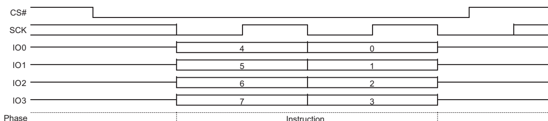
Figure 9.52 Erase or Program Resume Command Sequence QPI Mode
