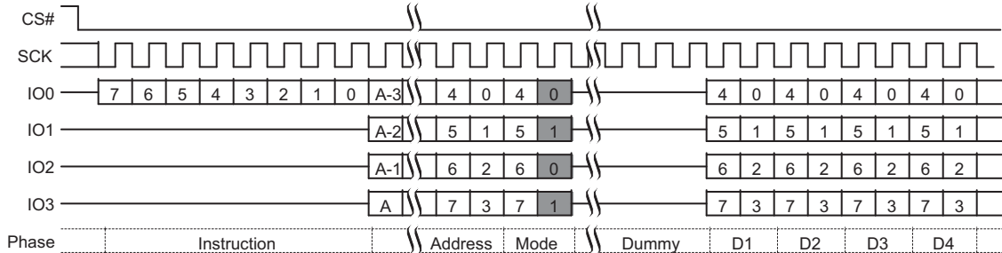
Figure 9.32 Quad I/O Read Command Sequence (EBh or ECh)
