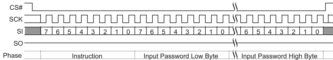
Figure 9.66 Password Unlock Command Sequence
