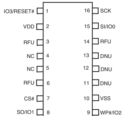
Figure 6.1 16-Lead SOIC Package (SO3016), Top View
