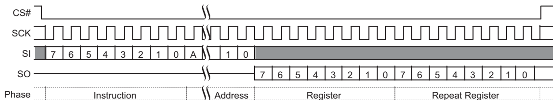
Figure 9.59 PPBRD Command Sequence
