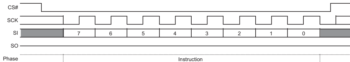
Figure 9.17 Clear Status Register (CLSR) Command Sequence
