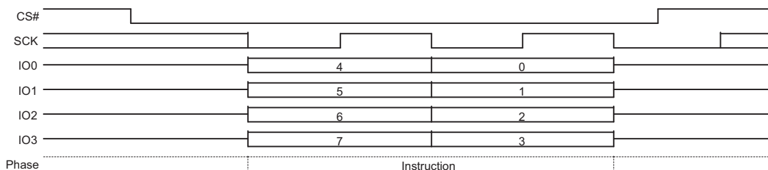
Figure 9.50 Program or Erase Suspend Command Sequence QPI Mode
