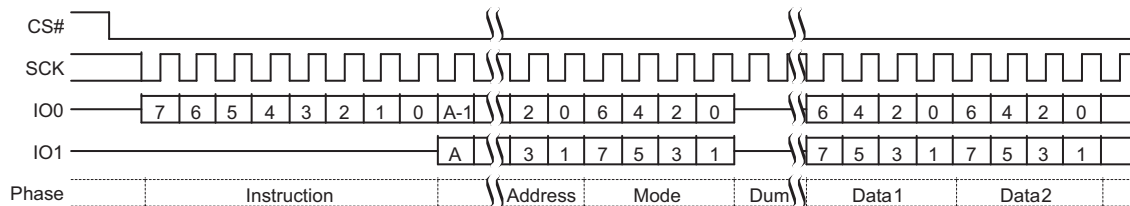
Figure 9.30 Dual I/O Read Command Sequence (BBh)
