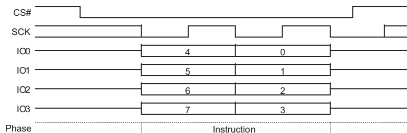
Figure 9.68 Software Reset Command Sequence QPI Mode
