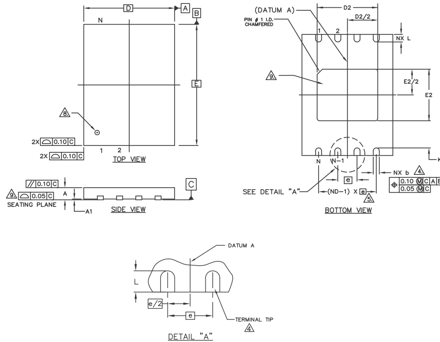
Figure 6.7 WSON 8-Contact 6x8 mm Leadless (WNH008)
