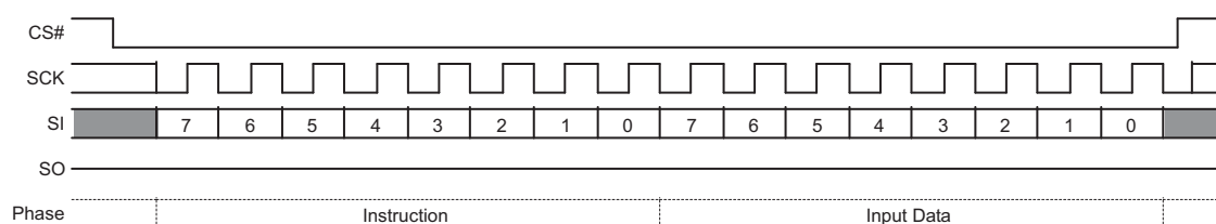
Figure 9.21 Program NVDLR (PNVDLR) Command Sequence
