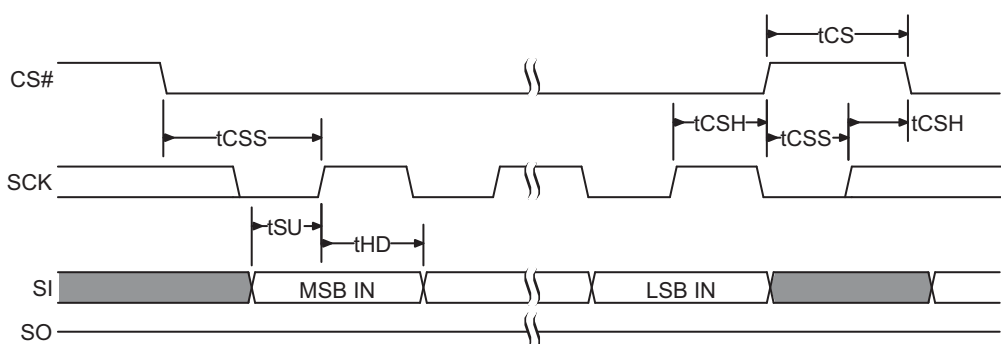
Figure 5.10 SPI Single Bit Input Timing
