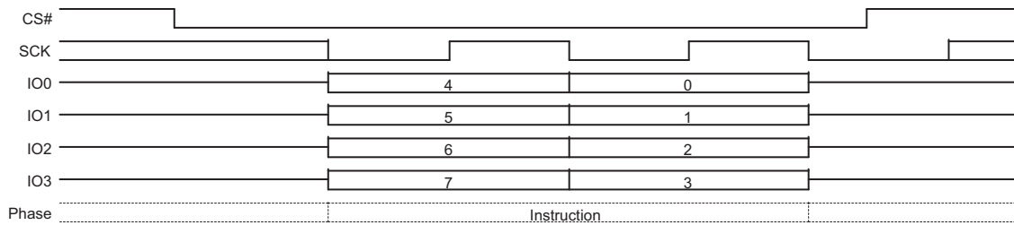
Figure 9.18 Clear Status Register (CLSR) Command Sequence QPI Mode
