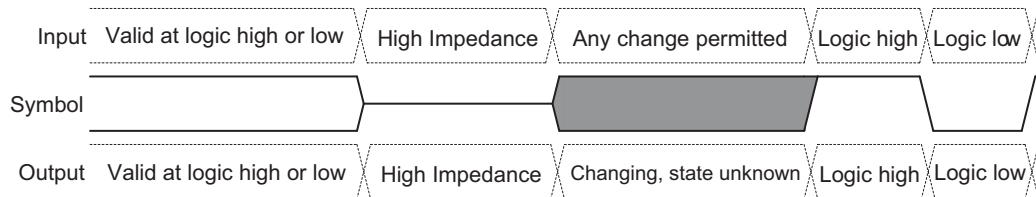
Figure 5.1 Waveform Element Meanings
