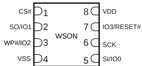
Figure 6.4 8-Connector Package (WSON 6x5), Top View
