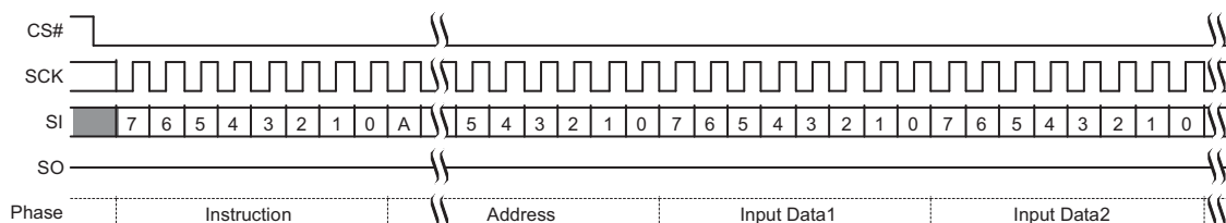
Figure 9.38 Page Program (PP 02h or 4PP 12h) Command Sequence
