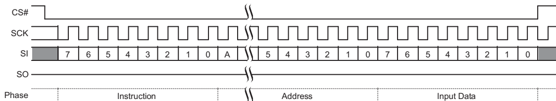
Figure 9.57 DYBWR Command Sequence
