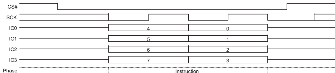
Figure 9.14 Write Enable (WREN) Command Sequence QPI Mode
