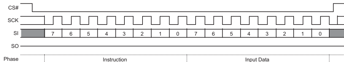
Figure 9.22 Write VDLR (WVDLR) Command Sequence
