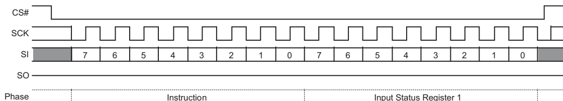
Figure 9.10 Write Registers (WRR) Command Sequence – 8-Data Bits
