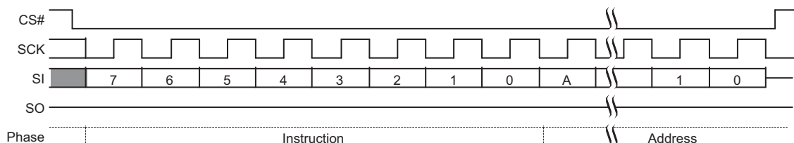
Figure 9.42 Sector Erase (SE D8h or 4SE DCh) Command Sequence
