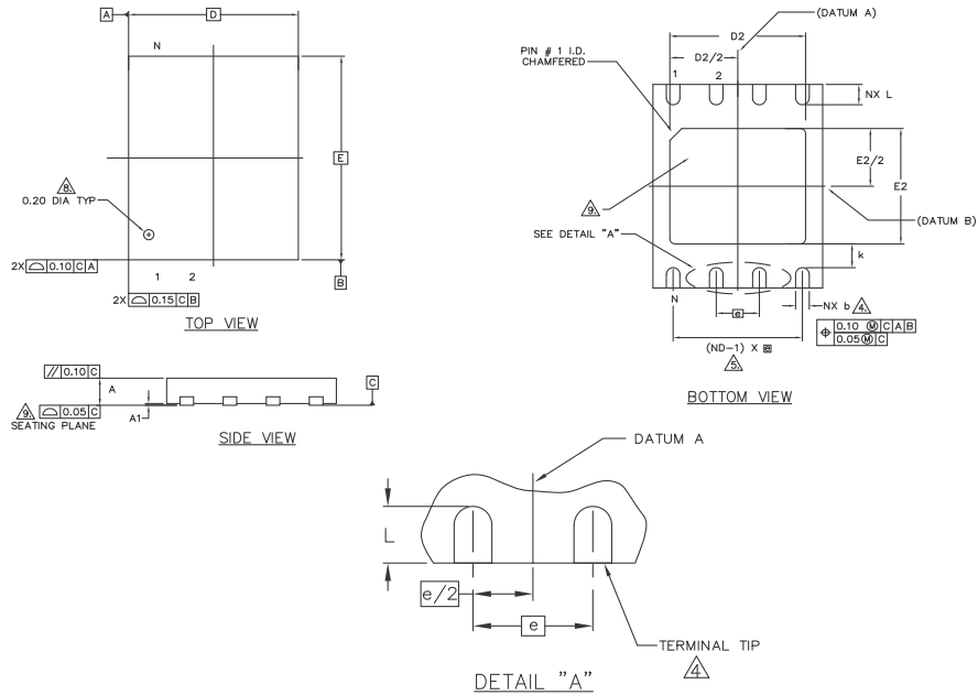
Figure 6.6 WSON 8-Contact 6x5 mm Leadless (WND008)
