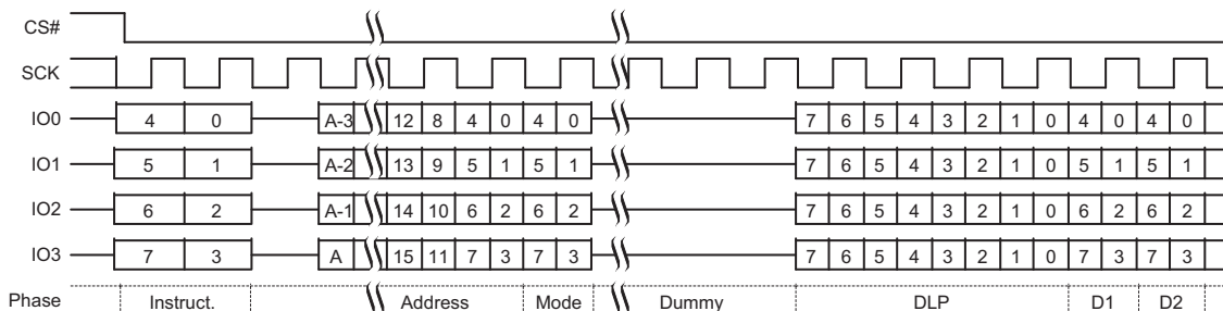
Figure 9.37 DDR Quad I/O Read Initial Access (EDh or EEh), QPI Mode
