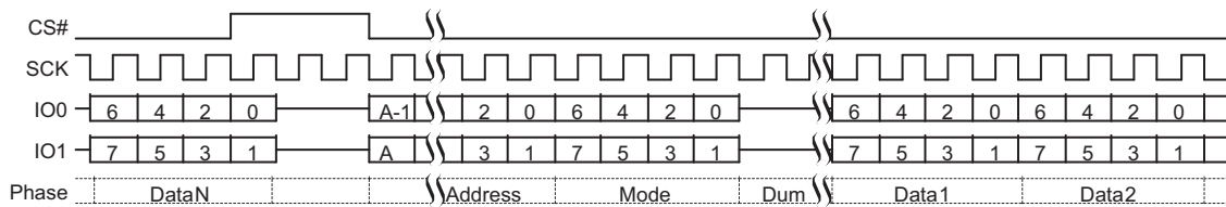
Figure 9.31 Dual I/O Continuous Read Command Sequence (4-Byte Address [CR2V[7] = 1])
