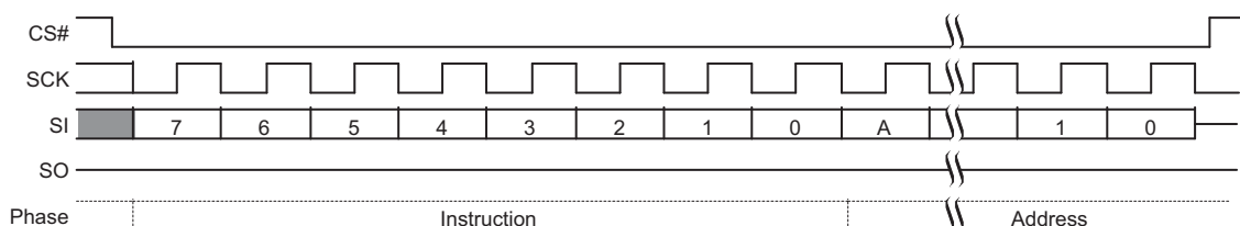
Figure 9.40 Parameter Sector Erase (P4E 20h or 4P4E 21h) Command Sequence
