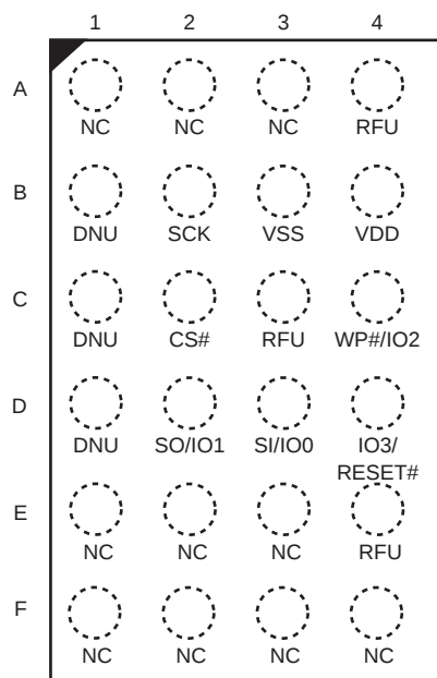
Figure 6.10 24-Ball BGA, 4x6 Ball Footprint (FAC024), Top View
