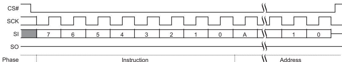
Figure 9.46 EES Command Sequence
