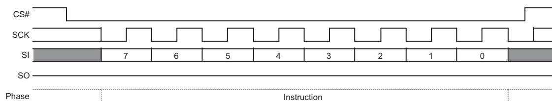
Figure 9.51 Erase or Program Resume Command Sequence
