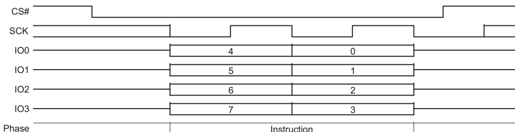
Figure 9.72 DPD Command Sequence QPI Mode
