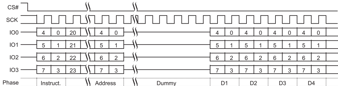
Figure 9.5 RSFDP QPI Mode Command Sequence
