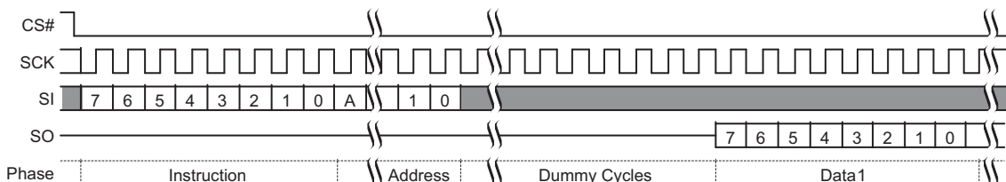
Figure 9.29 Fast Read (FAST_READ) Command Sequence (3-Byte Address, 0Bh [CR2V[7]=0])
