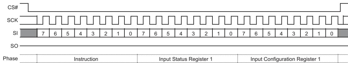
Figure 9.11 Write Registers (WRR) Command Sequence – 16-Data Bits
