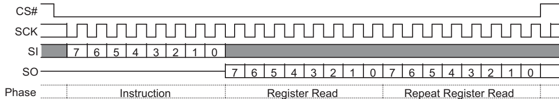
Figure 9.9 Read Configuration Register (RDCR) Command Sequence
