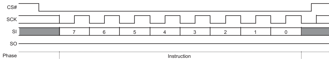
Figure 9.13 Write Enable (WREN) Command Sequence
