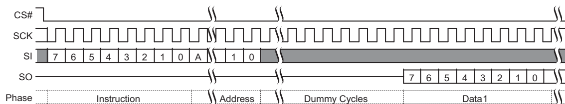
Figure 9.25 Read Any Register Read Command Sequence
