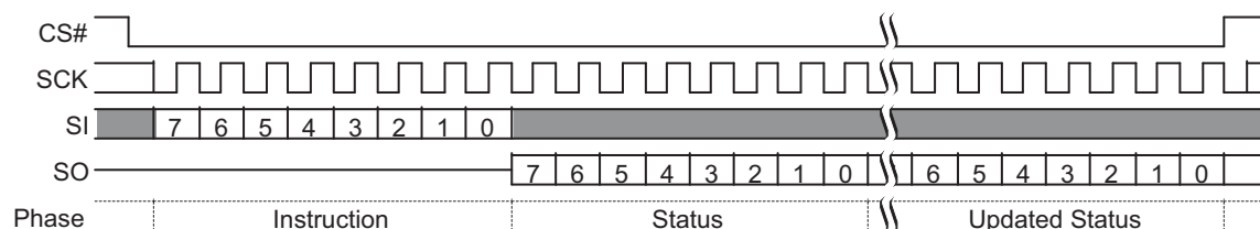
Figure 9.8 Read Status Register 2 (RDSR2) Command
