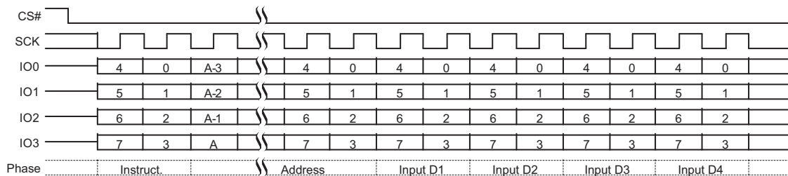
Figure 9.39 Page Program (PP 02h or 4PP 12h) QPI Mode Command Sequence
