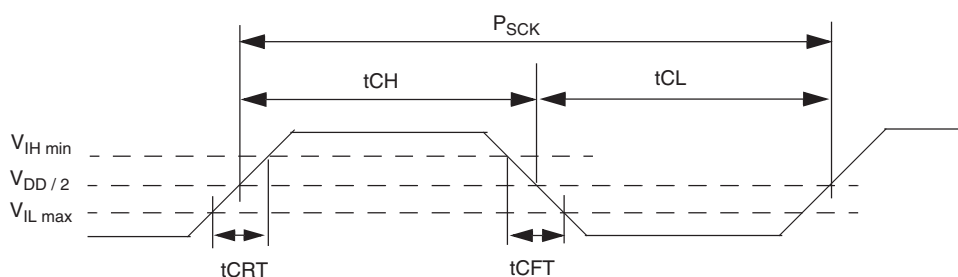
Figure 5.9 Clock Timing
