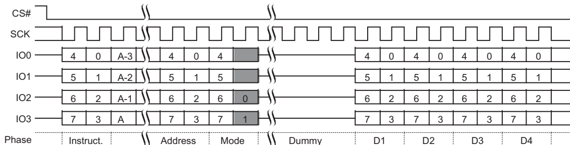
Figure 9.33 Quad I/O Read Command Sequence (EBh or ECh), QPI Mode
