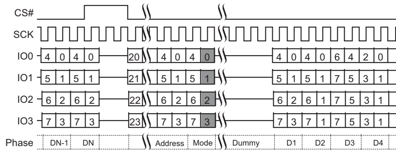
Figure 9.34 Continuous Quad I/O Read Command Sequence (3-Byte Address)
