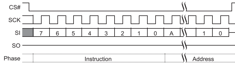
Figure 9.65 PPBP Command Sequence
