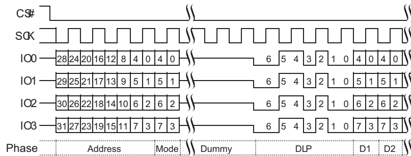
Figure 9.42 Continuous DDR Quad I/O Read Subsequent Access (4-Byte Address)
