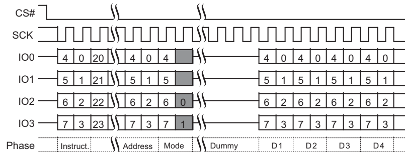
Figure 9.33 Quad I/O Read Command Sequence (3-Byte Address, EBh [CR2V[7]=0]) QPI Mode
