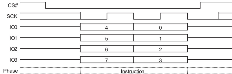
Figure 9.77 DPD Command Sequence QPI Mode
