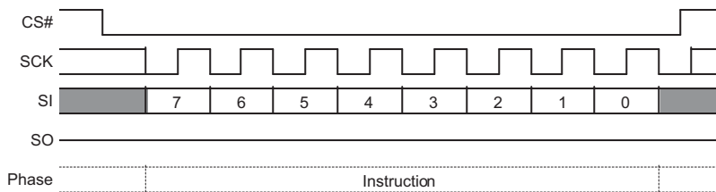
Figure 9.68 PPB Lock Bit Write Command Sequence
