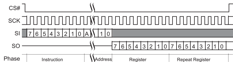
Figure 9.60 DYBRD Command Sequence
