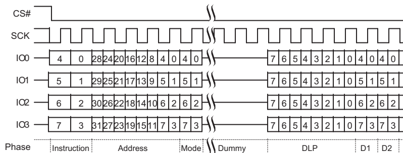
Figure 9.41 DDR Quad I/O Read Initial Access (4-Byte Address, EEh or EDh [CR2V[7]=1]) QPI Mode
