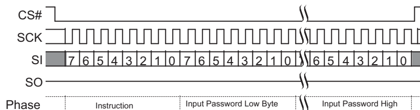
Figure 9.71 Password Unlock Command Sequence
