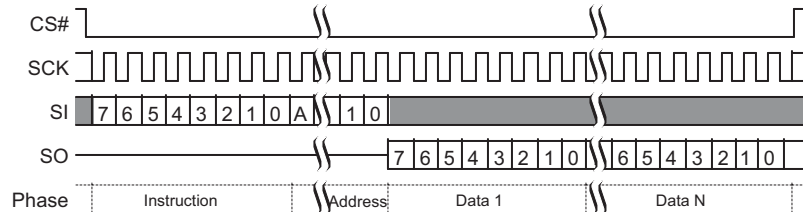
Figure 9.27 Read Command Sequence (3-Byte Address, 03h or 13h)
