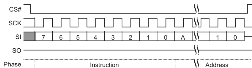
Figure 9.45 Parameter Sector Erase (P4E 20h or 4P4E 21h) Command Sequence
