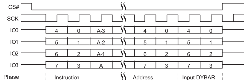
Figure 9.63 DYBWR QPI Mode Command Sequence
