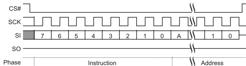
Figure 9.51 EES Command Sequence
