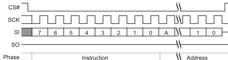
Figure 9.47 Sector Erase (SE D8h or 4SE DCh) Command Sequence
