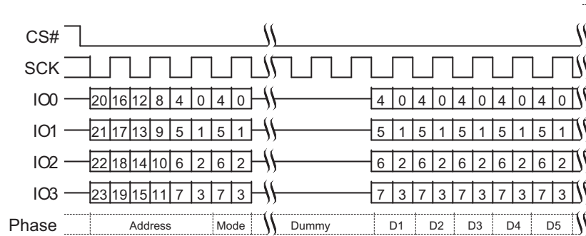
Figure 9.39 Continuous DDR Quad I/O Read Subsequent Access (3-Byte Address)
