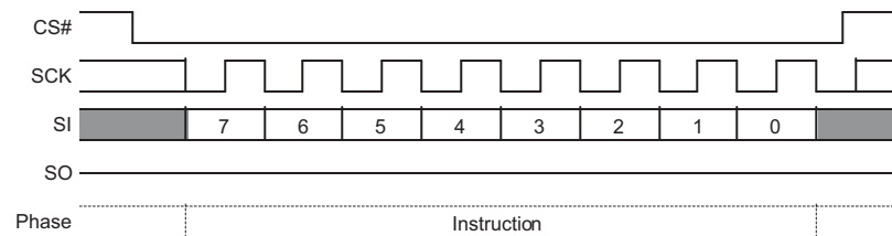
Figure 9.54 Erase or Program Suspend Command Sequence
