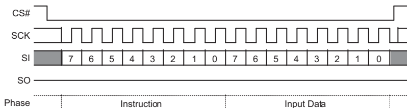
Figure 9.19 Program NVDLR (PNVDLR) Command Sequence
