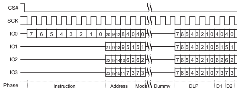
Figure 9.38 DDR Quad I/O Read Initial Access (3-Byte Address, EDh [CR2V[7]=0])
