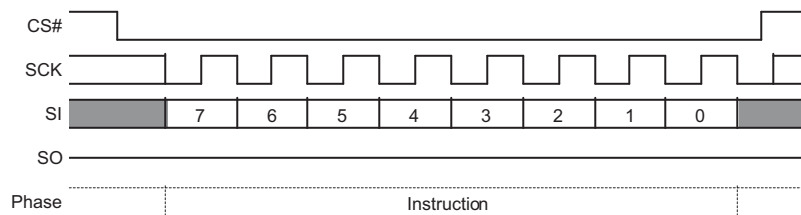
Figure 9.15 Write Disable (WRDI) Command Sequence
