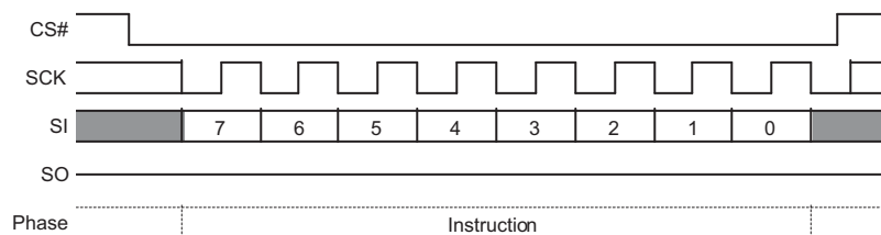
Figure 9.76 Deep Power-Down Command Sequence
