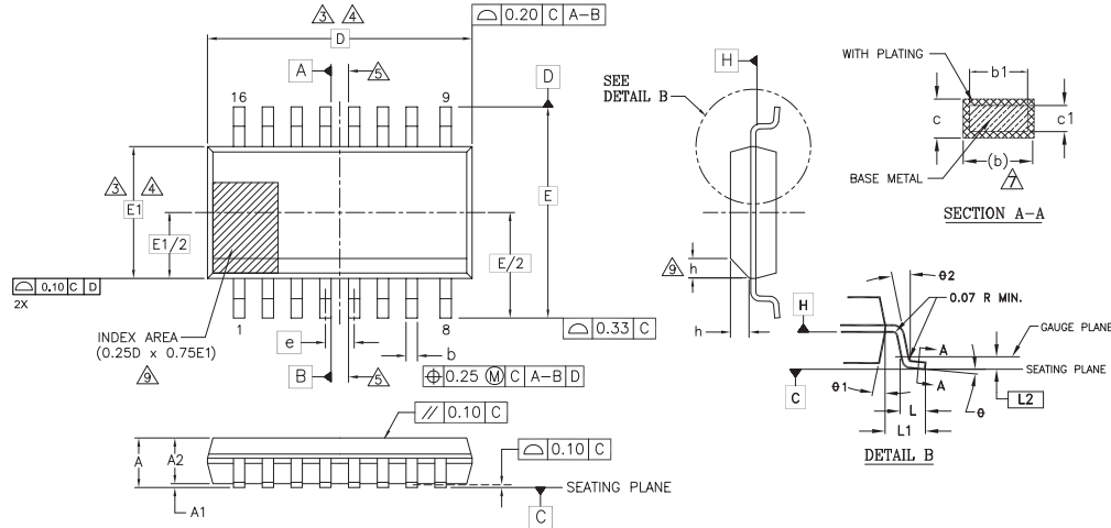
Figure 6.2 SOIC 16-Lead, 300-mil Body Width (SO3016)
