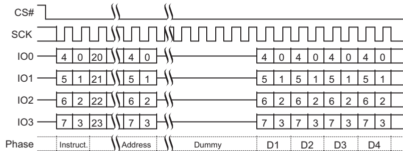
Figure 9.24 Read Any Register, QPI Mode, CR2[7] = 0, Command Sequence
