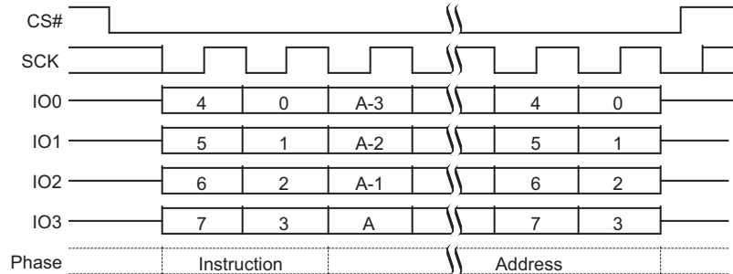
Figure 9.48 Sector Erase (SE D8h or 4SE DCh) QPI Mode Command Sequence
