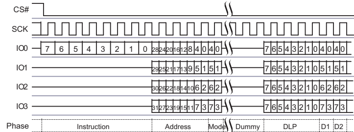
Figure 3.12 DDR Quad I/O Read in QPI Mode
