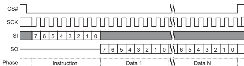
Figure 9.69 Password Read Command Sequence
