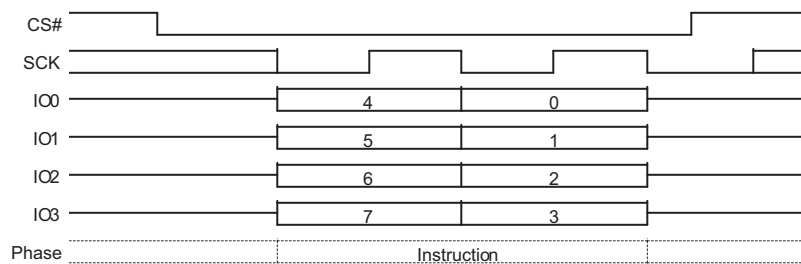
Figure 9.75 Mode Bit Reset Command Sequence QPI Mode
