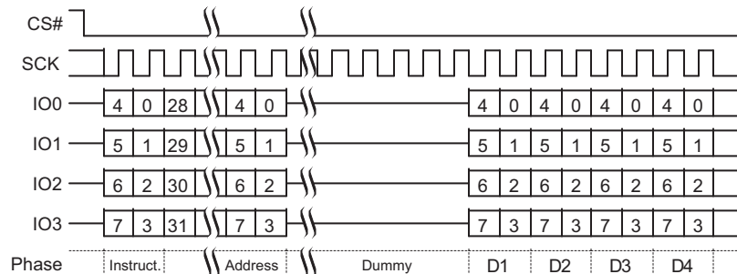
Figure 9.25 Read Any Register, QPI Mode, CR2[7] = 1 Command Sequence
