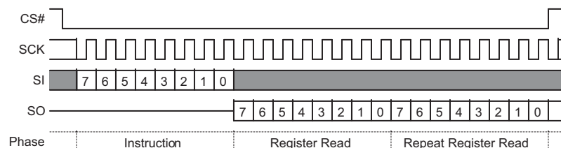
Figure 9.67 PPB Lock Register Read Command Sequence
