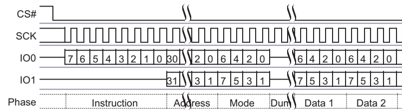
Figure 9.30 Dual I/O Read Command Sequence (4-Byte Address, BBh [CR2V[7]=1])
