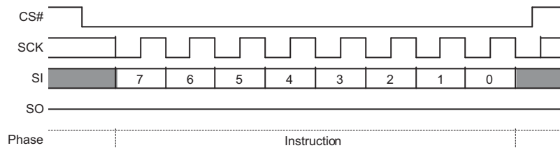
Figure 9.56 Erase or Program Resume Command Sequence
