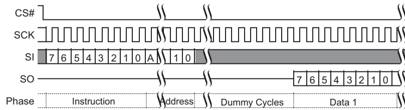
Figure 9.23 Read Any Register Read Command Sequence
