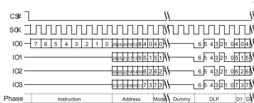
Figure 9.40 DDR Quad I/O Read Initial Access (4-Byte Address, EEh or EDh [CR2V[7]=1])
