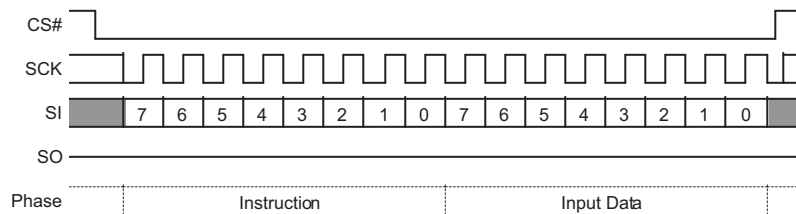
Figure 9.20 Write VDLR (WVDLR) Command Sequence
