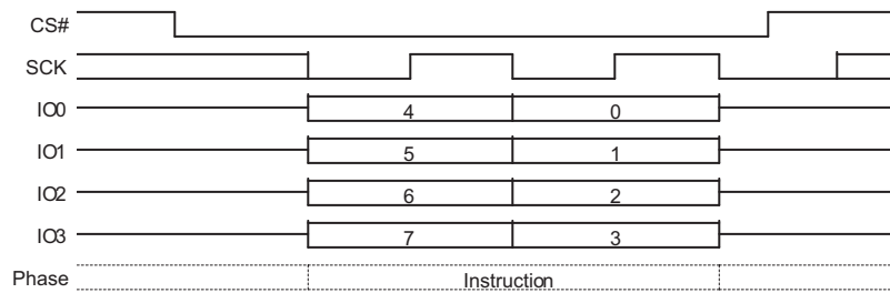
Figure 9.55 Erase or Program Suspend Command Sequence QPI Mode
