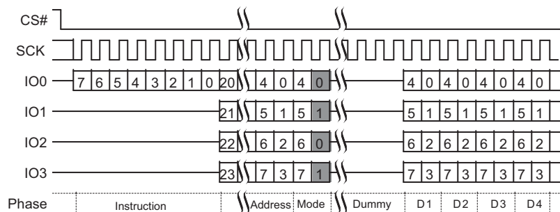
Figure 9.32 Quad I/O Read Command Sequence (3-Byte Address, EBh [CR2V[7]=0])
