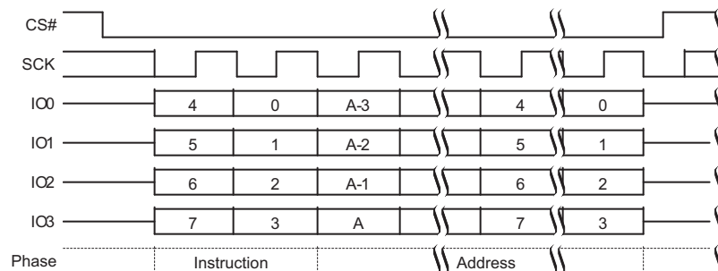
Figure 9.52 EES QPI Mode Command Sequence
