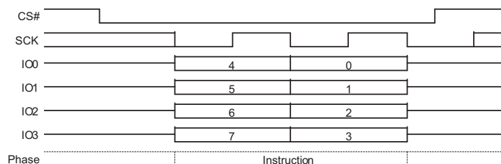
Figure 9.50 Bulk Erase Command Sequence QPI Mode
