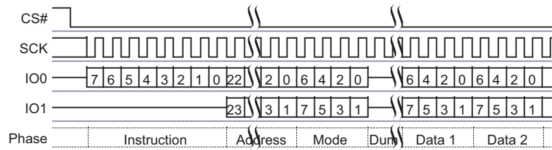
Figure 9.29 Dual I/O Read Command Sequence (3-Byte Address, BBh [CR2V[7]=0])
