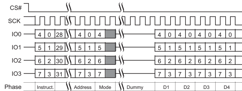
Figure 9.37 Quad I/O Read Command Sequence (4-Byte Address, ECh or EBh [CR2V[7]=1]) QPI Mode
