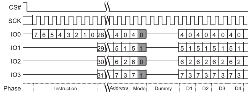
Figure 9.35 Quad I/O Read Command Sequence (4-Byte Address, ECh or EBh [CR2V[7]=1])
