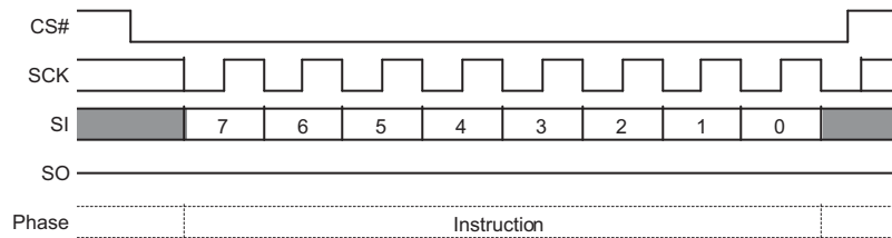
Figure 9.74 Mode Bit Reset Command Sequence
