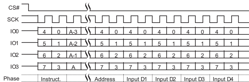
Figure 9.44 Page Program (PP 02h or 4PP 12h) QPI Mode Command Sequence
