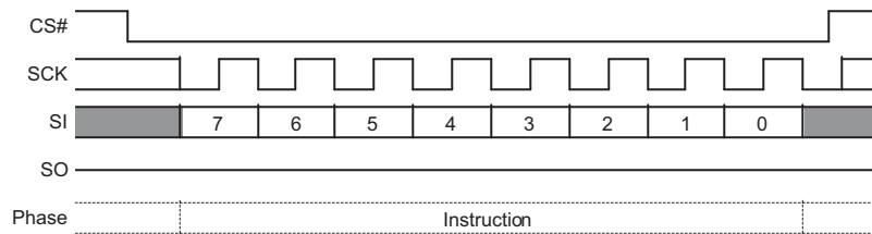
Figure 9.72 Software Reset Command Sequence
