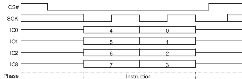
Figure 9.73 Software Reset Command Sequence QPI Mode
