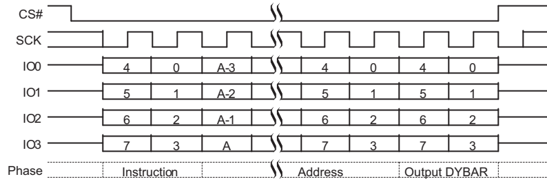
Figure 9.61 DYBRD QPI Mode Command Sequence
