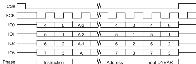
Figure 9.62 DYBWR Command Sequence
