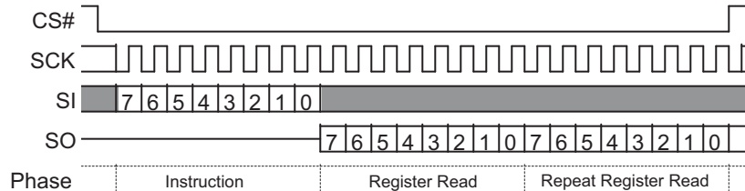
Figure 9.21 DLP Read (DLPRD) Command Sequence
