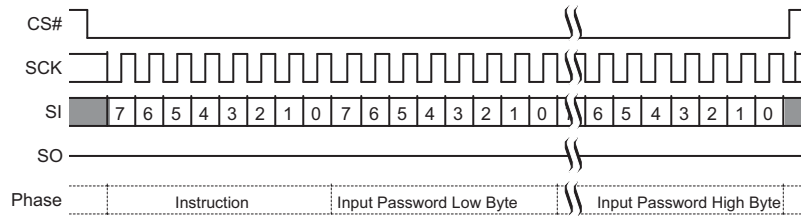
Figure 9.70 Password Program Command Sequence
