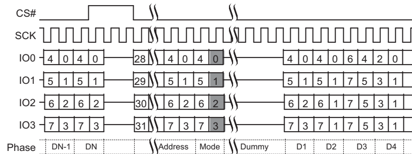
Figure 9.36 Continuous Quad I/O Read Command Sequence (4-Byte Address)
