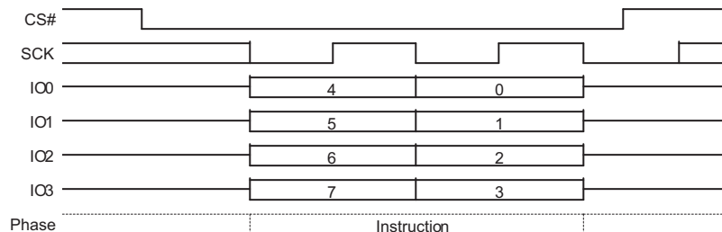
Figure 9.57 Erase or Program Resume Command Sequence QPI Mode
