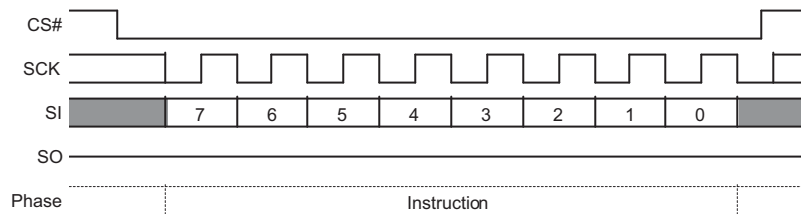
Figure 9.78 Release from Deep Power-Down Command Sequence
