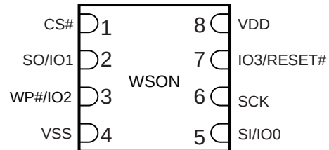
Figure 6.3 8-Connector Package (WSON 6x8), Top View
