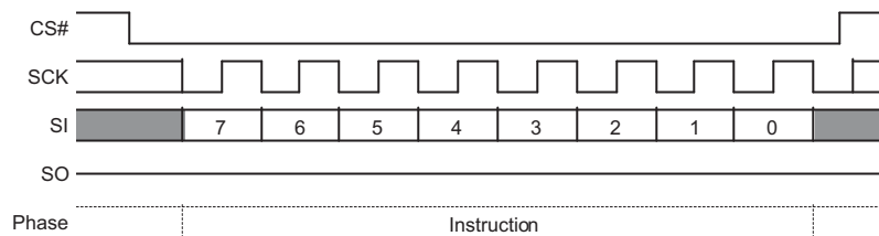
Figure 9.49 Bulk Erase Command Sequence
