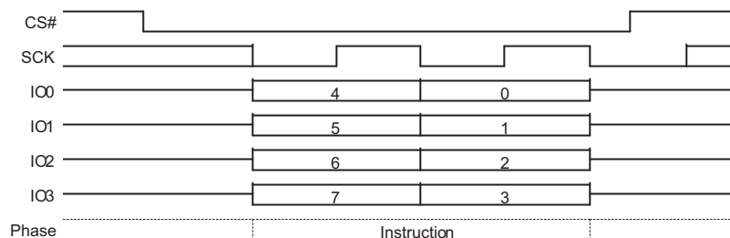
Figure 9.79 RES Command Sequence QPI Mode
