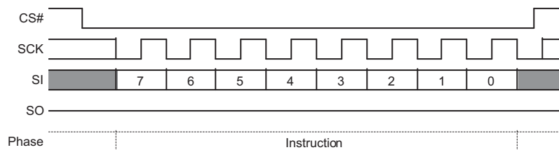
Figure 9.66 PPB Erase Command Sequence
