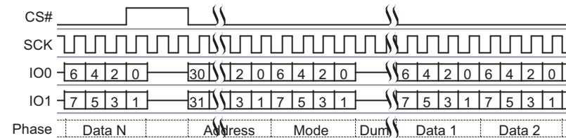
Figure 9.31 Dual I/O Continuous Read Command Sequence (4-Byte Address [CR2V[7]=1])
