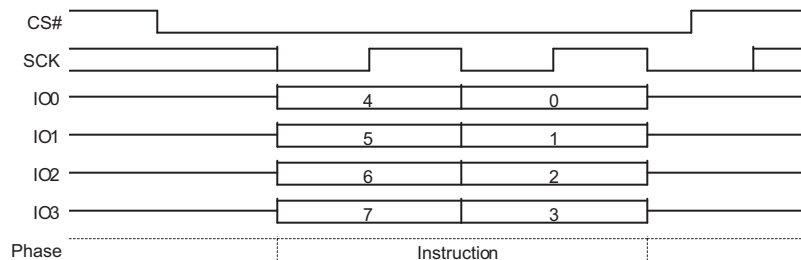
Figure 9.16 Write Disable (WRDI) Command Sequence QPI Mode
