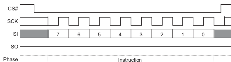
Figure 9.22 Enter 4-Byte Address Mode (4BAM B7h) Command Sequence
