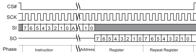
Figure 9.64 PPBRD Command Sequence
