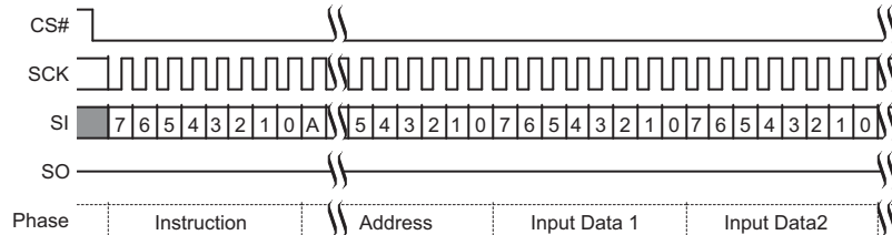
Figure 9.43 Page Program (PP 02h or 4PP 12h) Command Sequence
