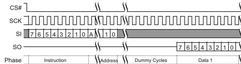
Figure 9.28 Fast Read (FAST_READ) Command Sequence (3-Byte Address, 0Bh [CR2V[7]=0])
