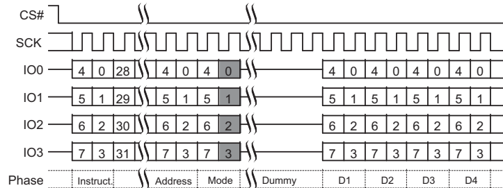
Figure 3.11 DDR Quad I/O Read
