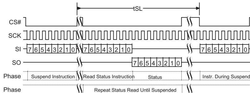
Figure 9.53 Program or Erase Suspend Command Sequence
