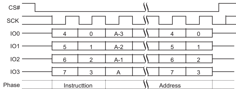
Figure 9.46 Parameter Sector Erase (P4E 20h or 4P4E 21h) QPI Mode Command Sequence
