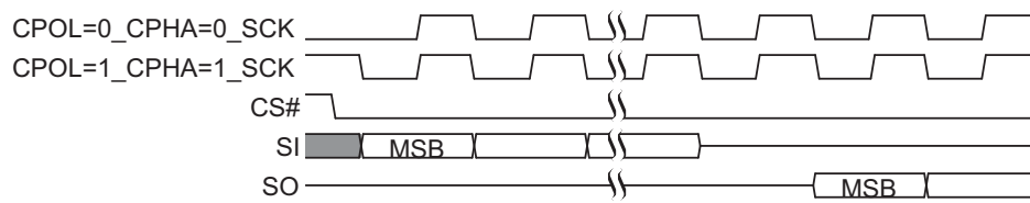
Figure 3.1 SPI SDR Modes Supported
