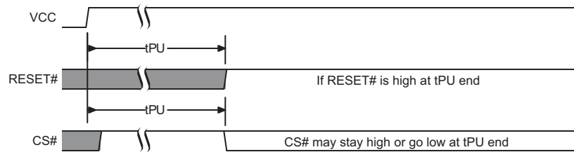
Figure 5.5 Reset High at the end of POR
