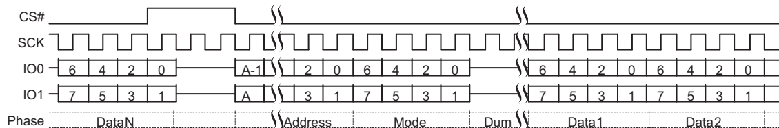
Figure 9.32 Dual I/O Continuous Read Command Sequence (BBh)
