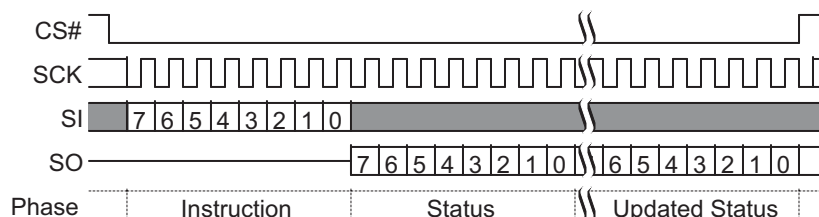
Figure 9.6 Read Status Register 1 (RDSR1) Command Sequence
