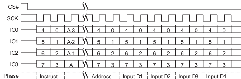
Figure 9.40 Page Program (PP 02h or 4PP 12h) QPI Mode Command Sequence
