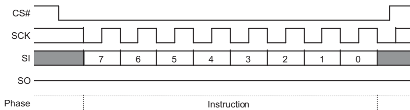
Figure 9.13 Write Enable (WREN) Command Sequence
