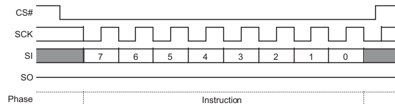
Figure 9.50 Erase or Program Suspend Command Sequence
