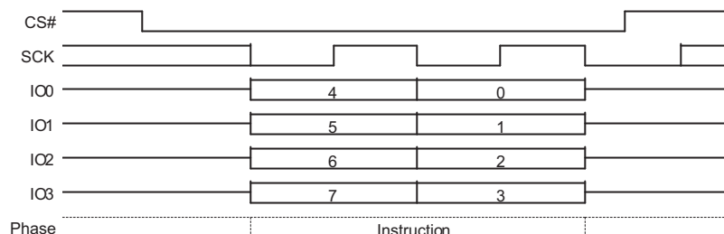
Figure 9.75 RES Command Sequence QPI Mode
