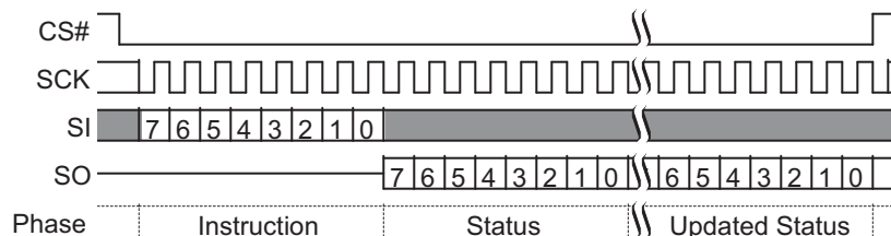
Figure 9.8 Read Status Register 2 (RDSR2) Command
