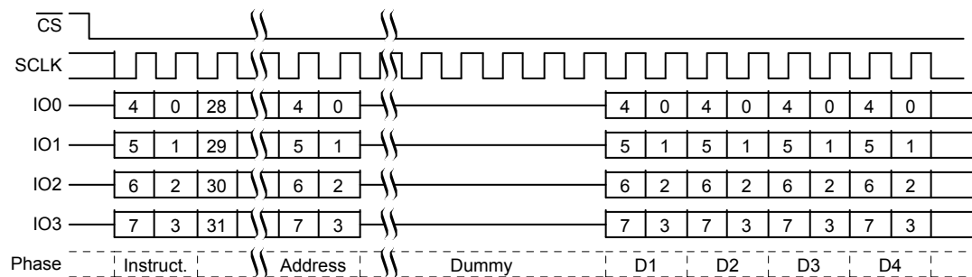
Figure 9.21 ECCRD (19h), QPI Mode, CR2[7] = 1, or 4ECCRD (18h) Command Sequence
