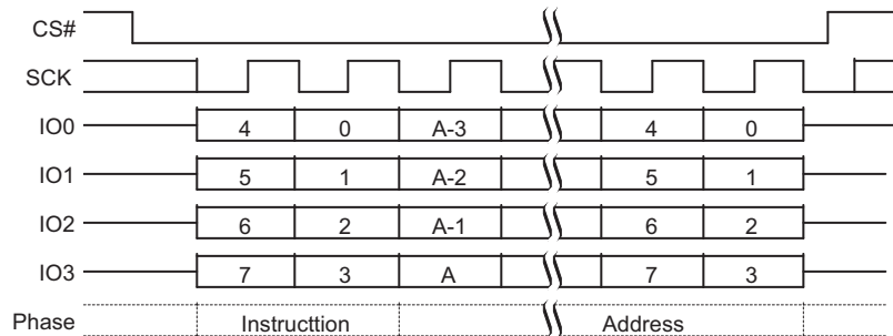
Figure 9.42 Parameter Sector Erase (P4E 20h or 4P4E 21h) QPI Mode Command Sequence
