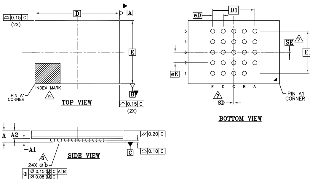
Figure 6.6 Ball Grid Array 24-Ball 6x8 mm (FAB024)
