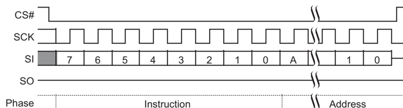
Figure 9.47 EES Command Sequence
