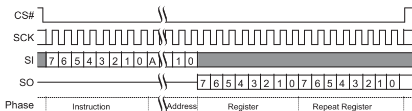
Figure 9.56 DYBRD Command Sequence
