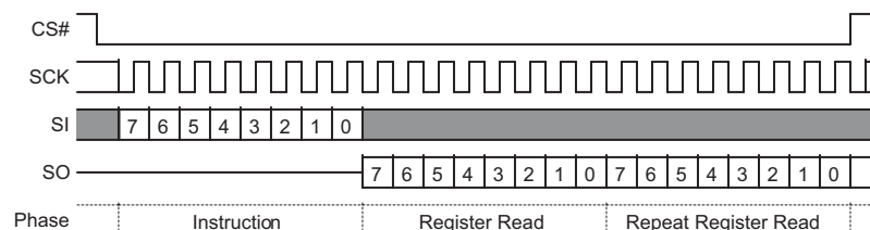
Figure 9.63 PPB Lock Register Read Command Sequence
