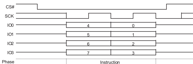
Figure 9.71 Mode Bit Reset Command Sequence QPI Mode
