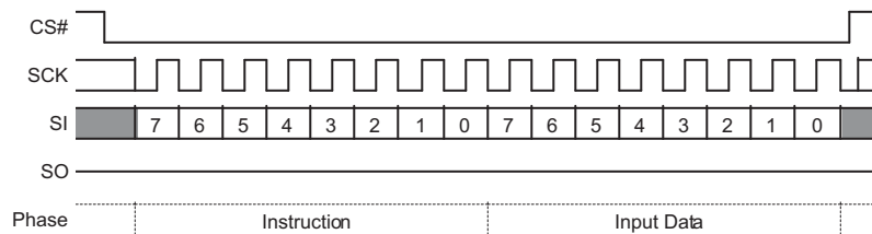
Figure 9.23 Write VDLR (WVDLR) Command Sequence
