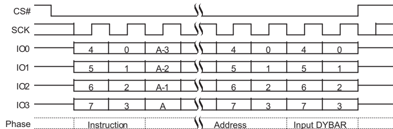
Figure 9.59 DYBWR QPI Mode Command Sequence
