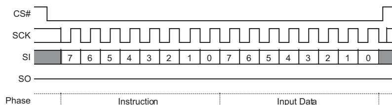
Figure 9.22 Program NVDLR (PNVDLR) Command Sequence
