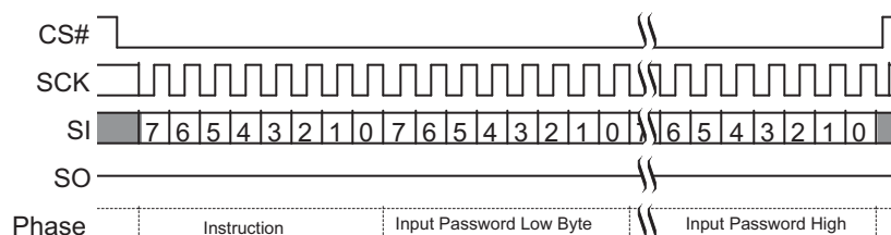
Figure 9.67 Password Unlock Command Sequence
