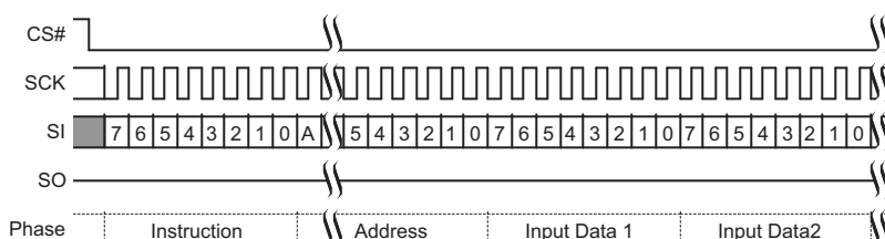
Figure 9.39 Page Program (PP 02h or 4PP 12h) Command Sequence
