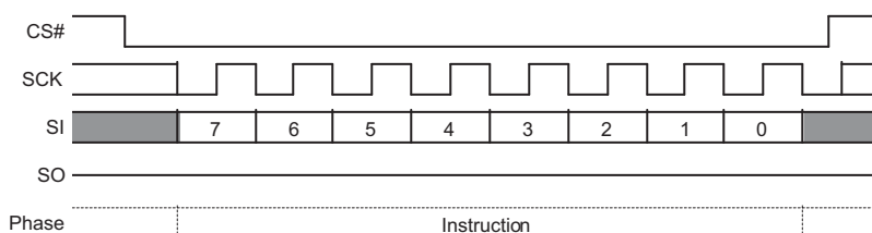
Figure 9.72 Deep Power-Down Command Sequence
