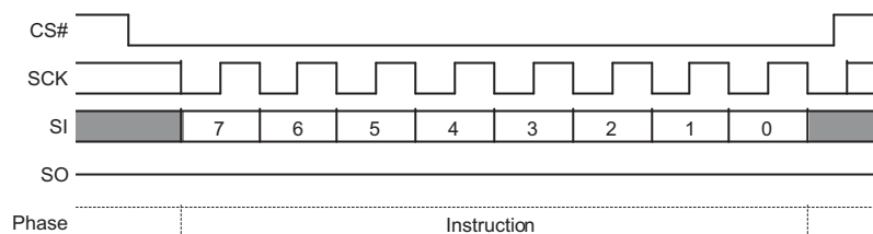
Figure 9.45 Bulk Erase Command Sequence
