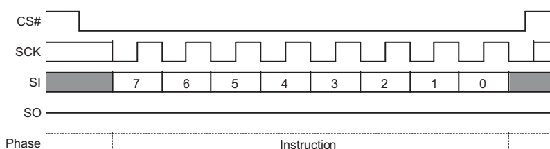
Figure 9.15 Write Disable (WRDI) Command Sequence
