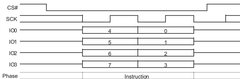
Figure 9.18 Clear Status Register (CLSR) Command Sequence QPI Mode
