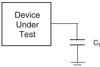
Figure 5.2 Test Setup
