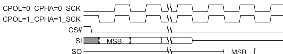
Figure 3.1 SPI SDR Modes Supported
