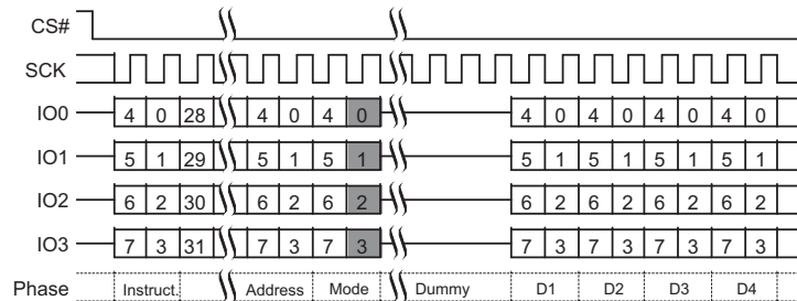
Figure 3.11 DDR Quad I/O Read
