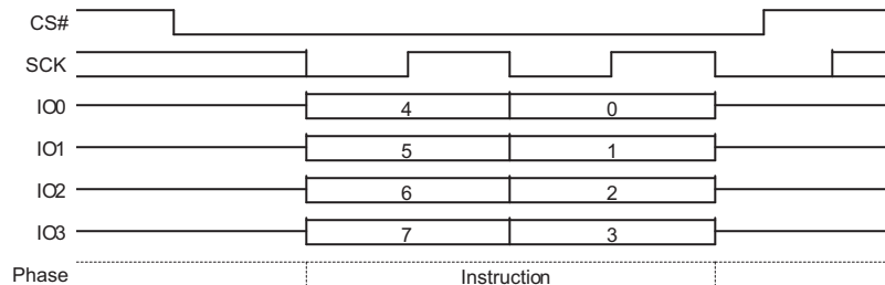
Figure 9.73 DPD Command Sequence QPI Mode
