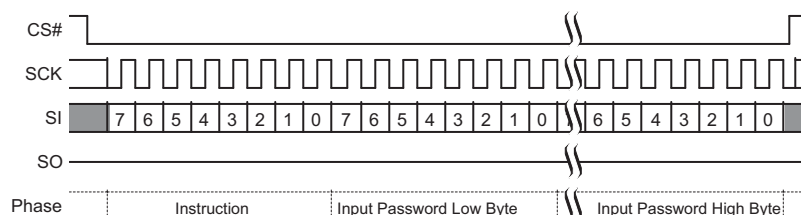
Figure 9.66 Password Program Command Sequence
