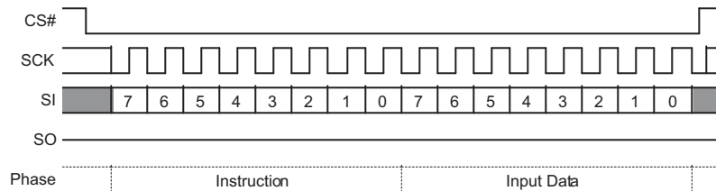
Figure 9.28 Set Burst Length Command Sequence
