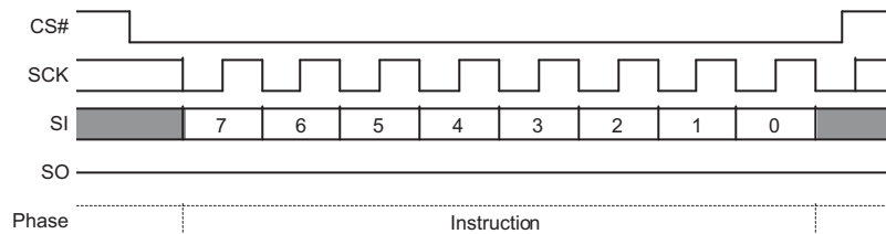
Figure 9.52 Erase or Program Resume Command Sequence
