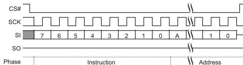
Figure 9.43 Sector Erase (SE D8h or 4SE DCh) Command Sequence
