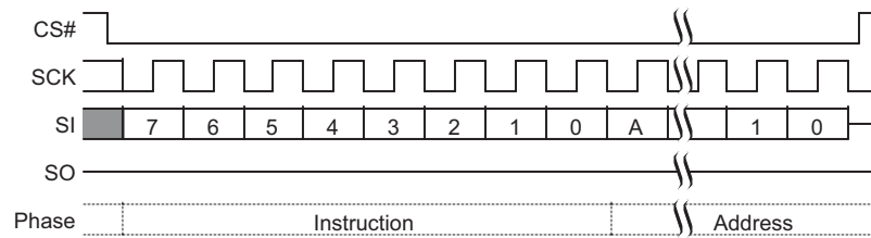
Figure 9.61 PPBP Command Sequence
