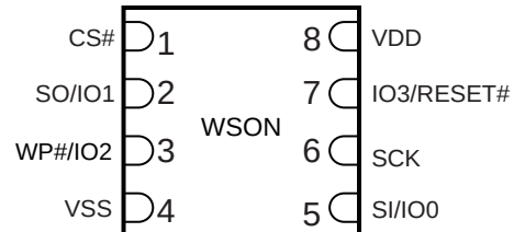
Figure 6.3 8-Connector Package (WSO6 6x8), Top View
