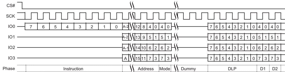
Figure 9.36 DDR Quad I/O Read Initial Access (EDh or EEh)
