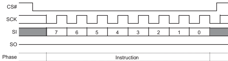
Figure 9.17 Clear Status Register (CLSR) Command Sequence
