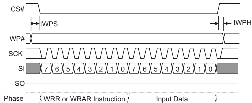
Figure 5.13 WP# Input Timing
