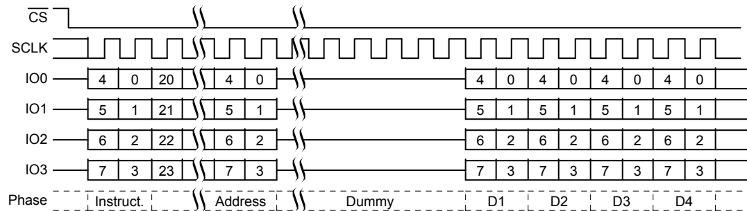
Figure 9.20 ECCRD (19h), QPI Mode, CR2[7] = 0, Command Sequence
