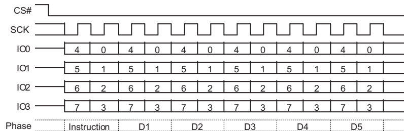
Figure 9.3 Read Quad Identification (RDQID) Command Sequence
