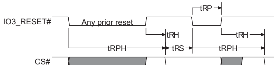
Figure 5.7 Hardware Reset when Quad Mode is not Enabled and IO3 / Reset# is Enabled
