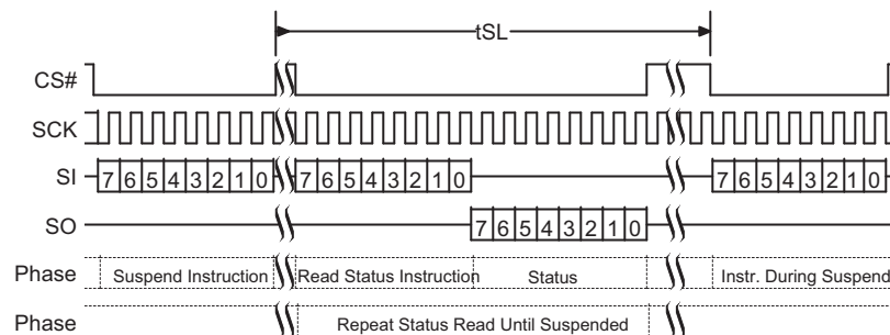
Figure 9.49 Program or Erase Suspend Command Sequence
