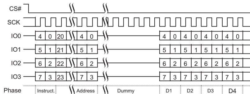
Figure 9.5 RSFDP QPI Mode Command Sequence
