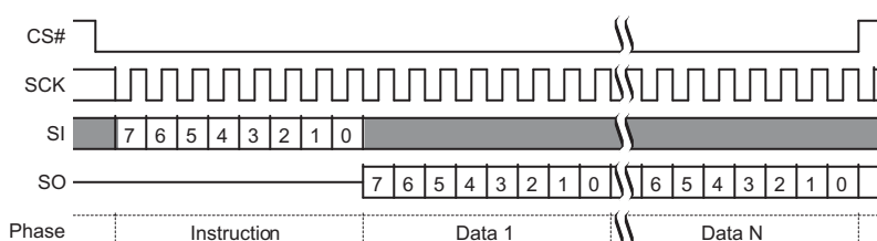
Figure 9.65 Password Read Command Sequence
