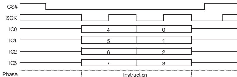
Figure 9.14 Write Enable (WREN) Command Sequence QPI Mode
