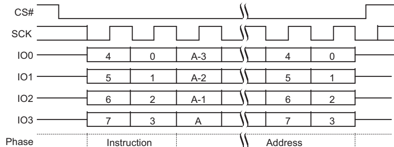
Figure 9.44 Sector Erase (SE D8h or 4SE DCh) QPI Mode Command Sequence
