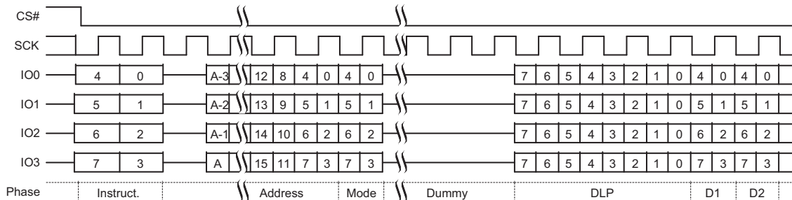
Figure 9.38 DDR Quad I/O Read Initial Access (EDh or EEh), QPI Mode
