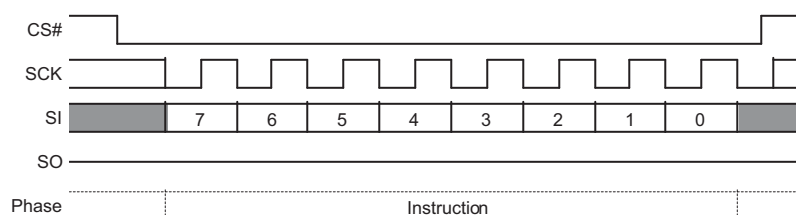
Figure 9.25 Enter 4-Byte Address Mode (4BAM B7h) Command Sequence
