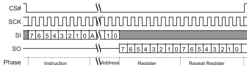
Figure 9.60 PPBRD Command Sequence
