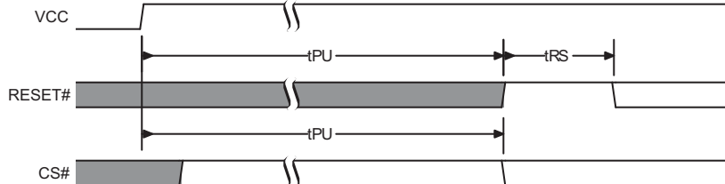
Figure 5.6 POR followed by Hardware Reset
