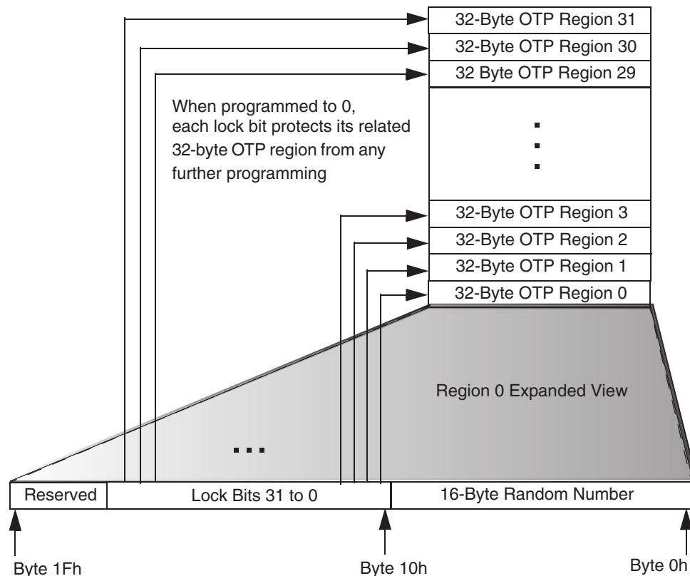
Figure 7.1 OTP Address Space
