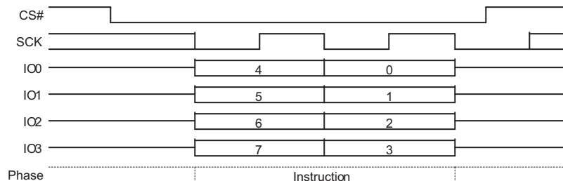
Figure 9.53 Erase or Program Resume Command Sequence QPI Mode
