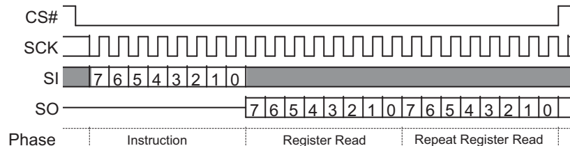
Figure 9.24 DLP Read (DLPRD) Command Sequence
