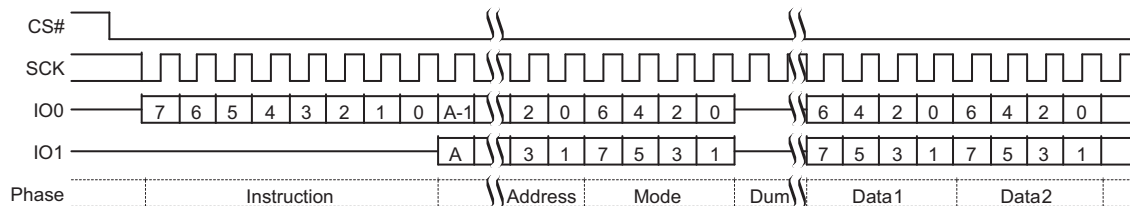
Figure 9.31 Dual I/O Read Command Sequence (BBh)
