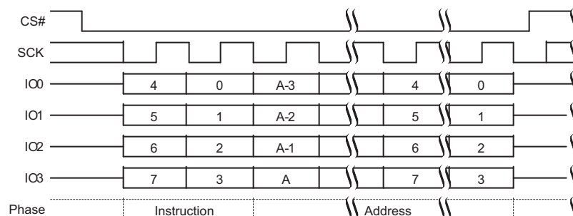
Figure 9.48 EES QPI Mode Command Sequence
