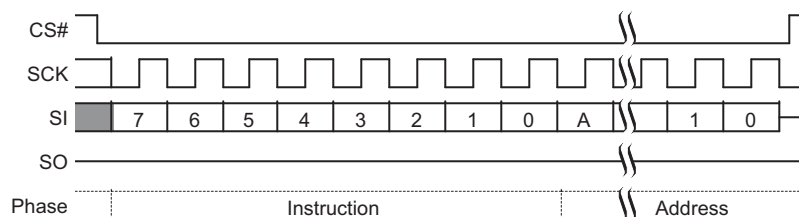
Figure 9.41 Parameter Sector Erase (P4E 20h or 4P4E 21h) Command Sequence
