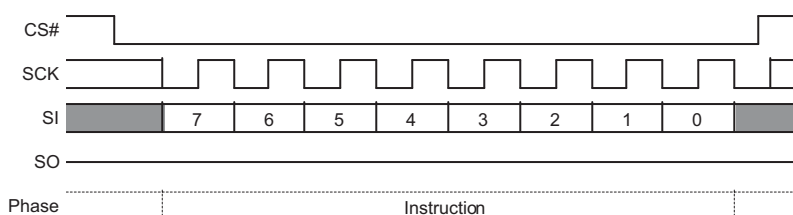
Figure 9.64 PPB Lock Bit Write Command Sequence
