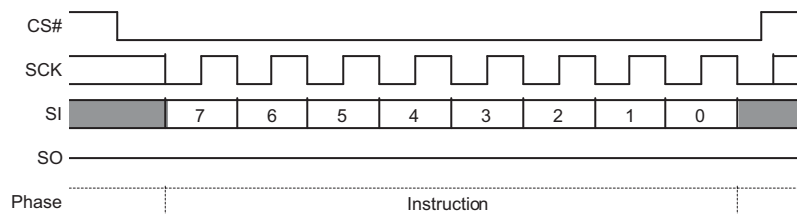
Figure 9.62 PPB Erase Command Sequence
