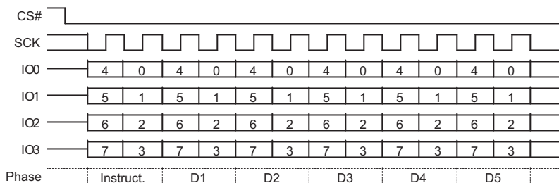
Figure 9.7 Read Status Register 1 (RDSR1) QPI Mode Command
