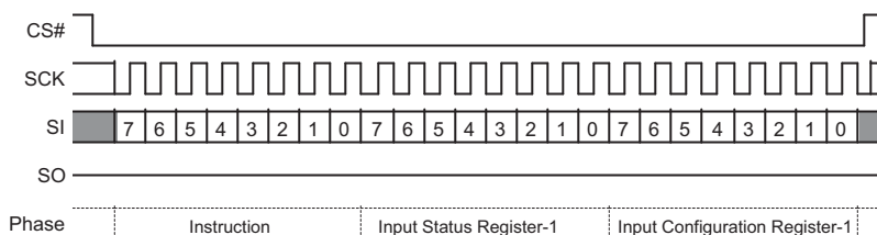
Figure 9.11 Write Registers (WRR) Command Sequence – 16 Data Bits
