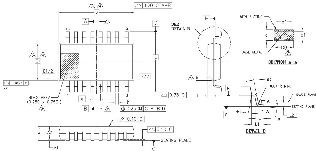
Figure 6.2 SOIC 16-Lead, 300-mil Body Width (SO3016)
