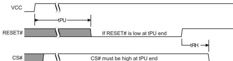
Figure 5.4 Reset Low at the end of POR
