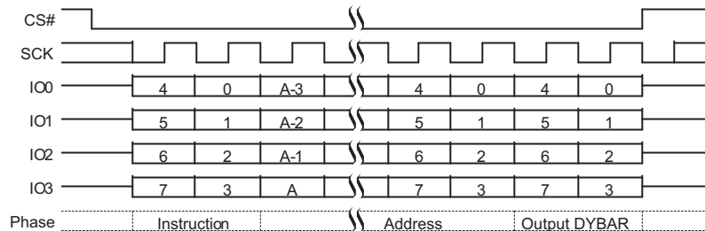
Figure 9.57 DYBRD QPI Mode Command Sequence
