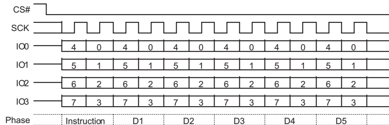
Figure 9.2 Read Identification (RDID) QPI Mode Command
