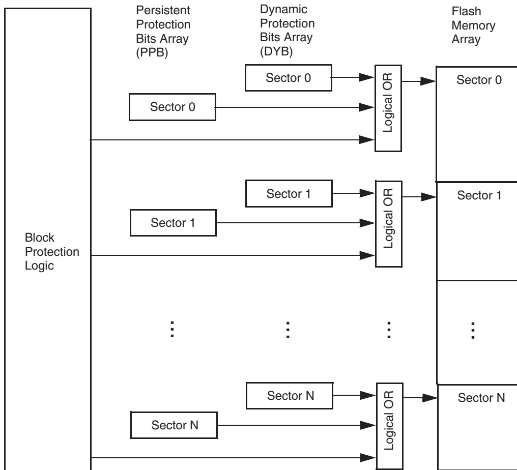
Figure 8.1 Sector Protection Control
