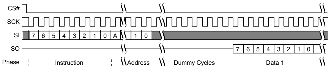
Figure 9.19 ECC Status Register Read Command Sequence
