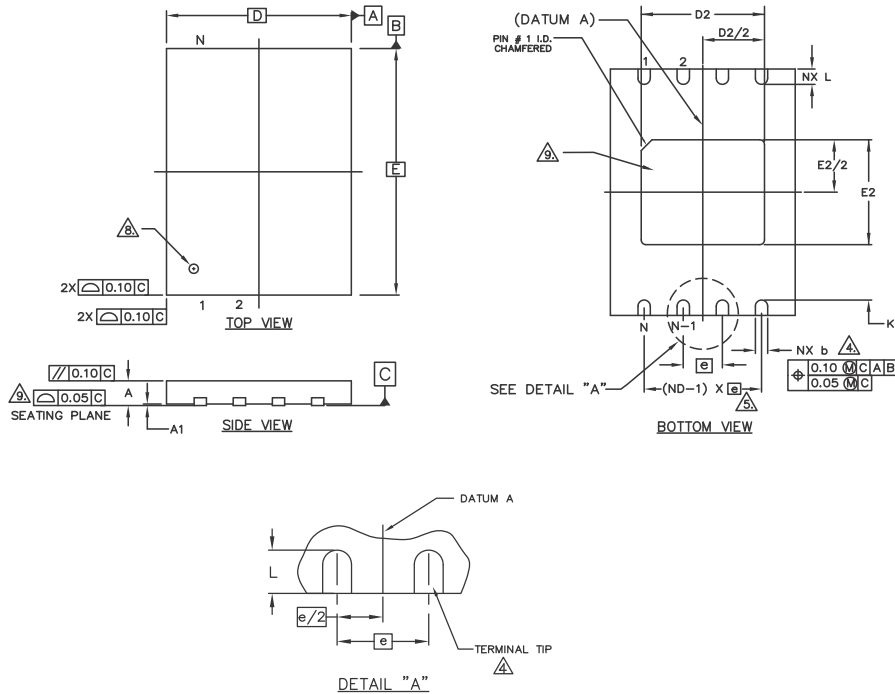
Figure 6.4 WSON 8-Contact 6x8 mm Leadless (WNH008)
