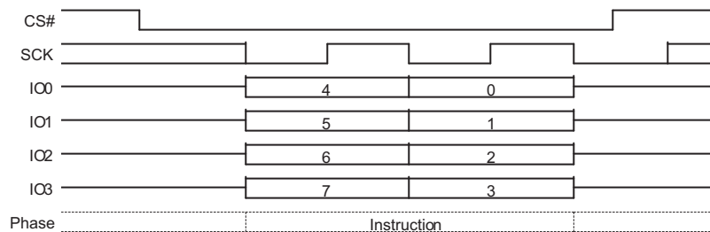
Figure 9.69 Software Reset Command Sequence QPI Mode
