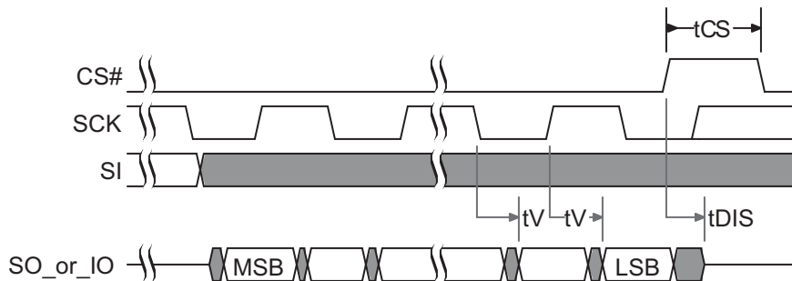
Figure 5.15 SPI DDR Output Timing
