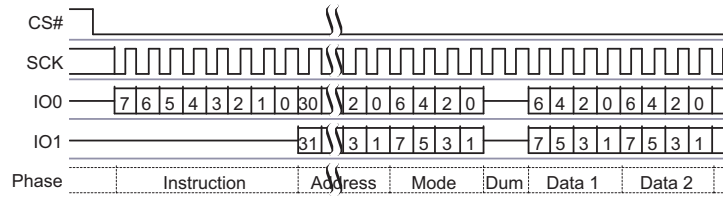
Figure 3.9 Quad I/O Command
