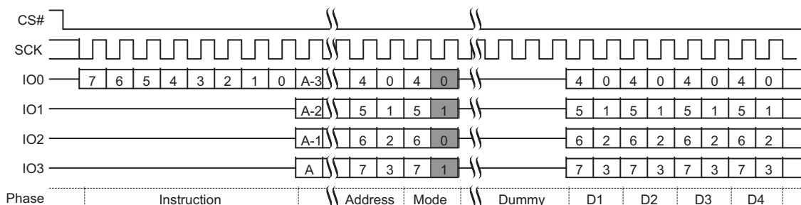
Figure 9.33 Quad I/O Read Command Sequence (EBh or ECh)
