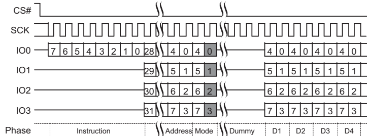
Figure 3.10 Quad I/O Read Command in QPI Mode
