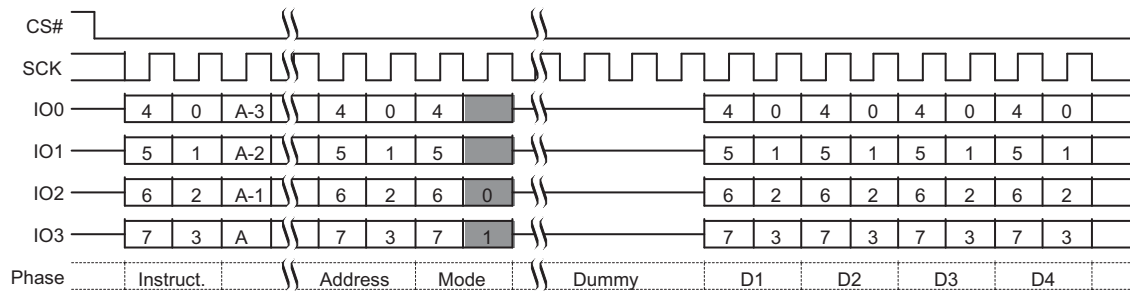
Figure 9.34 Quad I/O Read Command Sequence (EBh or ECh), QPI Mode
