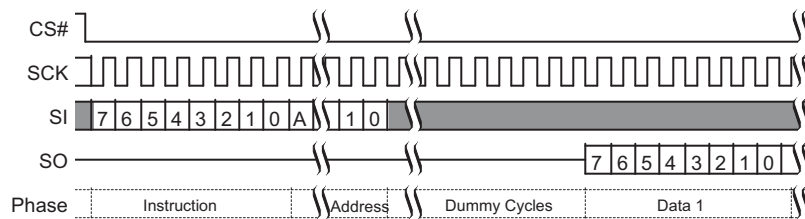
Figure 9.30 Fast Read (FAST_READ) Command Sequence (3-Byte Address, 0Bh [CR2V[7]=0])
