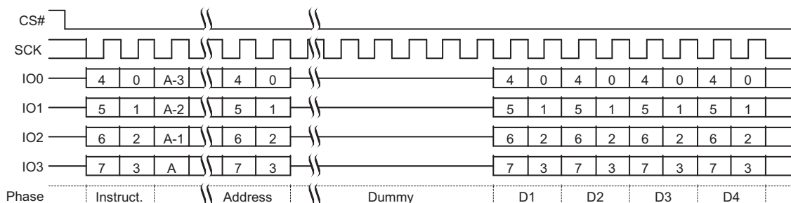
Figure 9.27 Read Any Register, QPI Mode, Command Sequence
