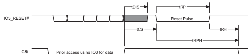
Figure 5.8 Hardware Reset when Quad Mode and IO3 / Reset# are Enabled
