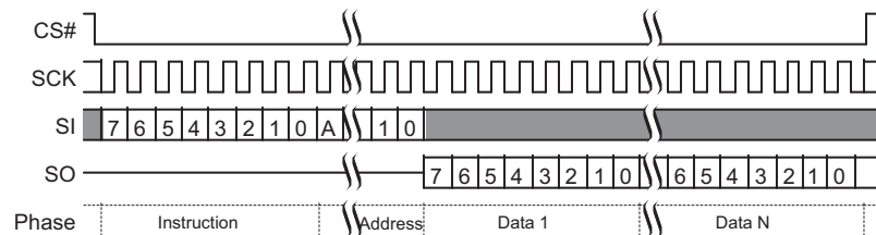
Figure 9.29 Read Command Sequence (3-Byte Address, 03h or 13h)
