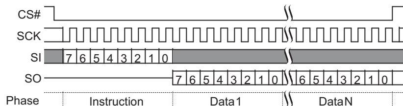
Figure 9.1 Read Identification (RDID) Command Sequence
