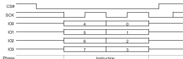
Figure 9.46 Bulk Erase Command Sequence QPI Mode
