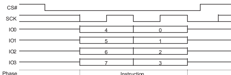
Figure 9.16 Write Disable (WRDI) Command Sequence QPI Mode
