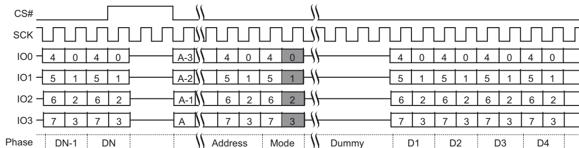
Figure 9.35 Continuous Quad I/O Read Command Sequence (EBh or ECh)
