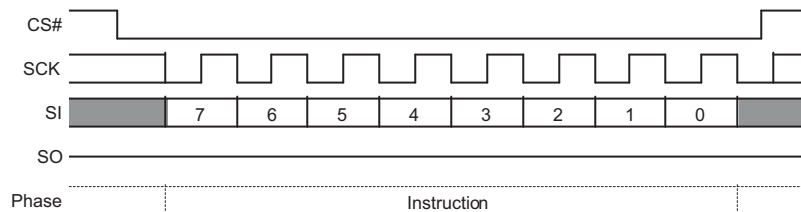
Figure 9.74 Release from Deep Power-Down Command Sequence
