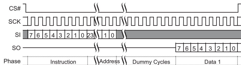
Figure 9.4 RSFDP Command Sequence
