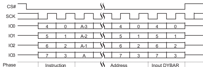
Figure 9.58 DYBWR Command Sequence
