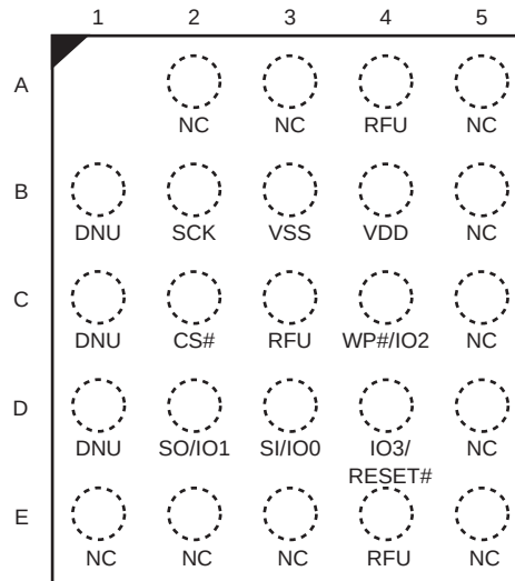
Figure 6.5 24-Ball BGA, 5x5 Ball Footprint (FAB024), Top View
