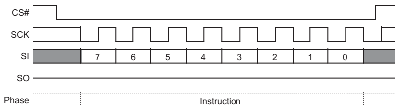
Figure 9.70 Mode Bit Reset Command Sequence
