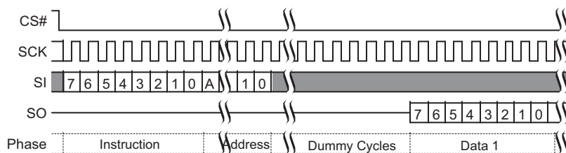
Figure 9.26 Read Any Register Read Command Sequence
