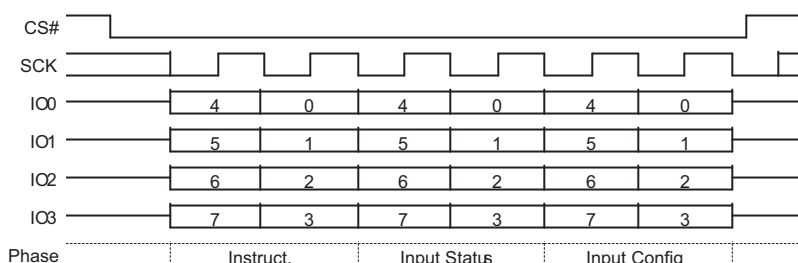
Figure 9.12 Write Registers (WRR) Command Sequence – 16 Data Bits QPI Mode
