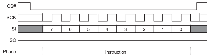
Figure 9.68 Software Reset Command Sequence
