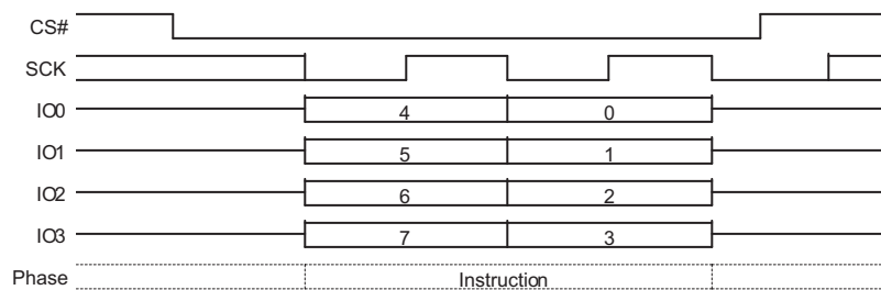
Figure 9.51 Erase or Program Suspend Command Sequence QPI Mode
