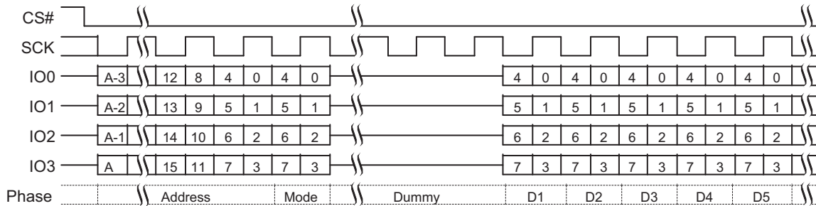
Figure 9.37 Continuous DDR Quad I/O Read Subsequent Access (EDh or EEh)
