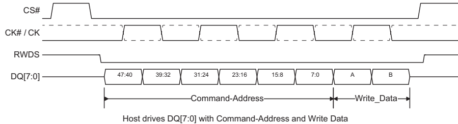
Figure 9. Write Operation
